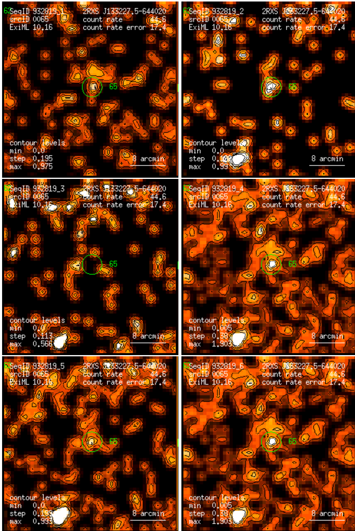
Figure 65: RASS 932819: detection 0065: band rate images, Gaussian filter: (1) PSPC channels 11 – 41, (2) 52 – 90, (3) 91 – 201, (4) 11 – 235, (5) 52 – 201, (6) 11 – 201. Broad band rates in counts/ks. Band rate contour levels in counts/ks/arcmin 2 .
