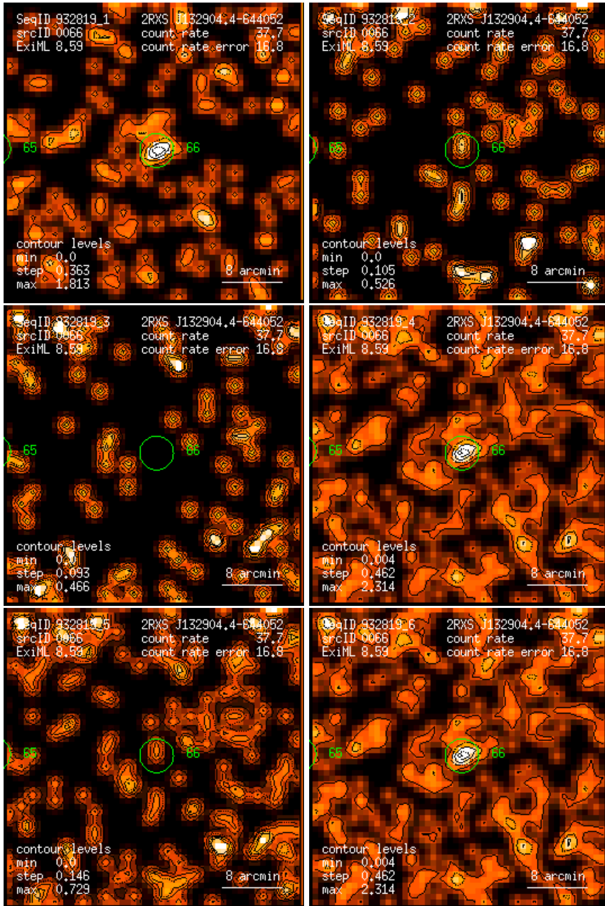
Figure 66: RASS 932819: detection 0066: band rate images, Gaussian filter: (1) PSPC channels 11 – 41, (2) 52 – 90, (3) 91 – 201, (4) 11 – 235, (5) 52 – 201, (6) 11 – 201. Broad band rates in counts/ks. Band rate contour levels in counts/ks/arcmin 2 .
