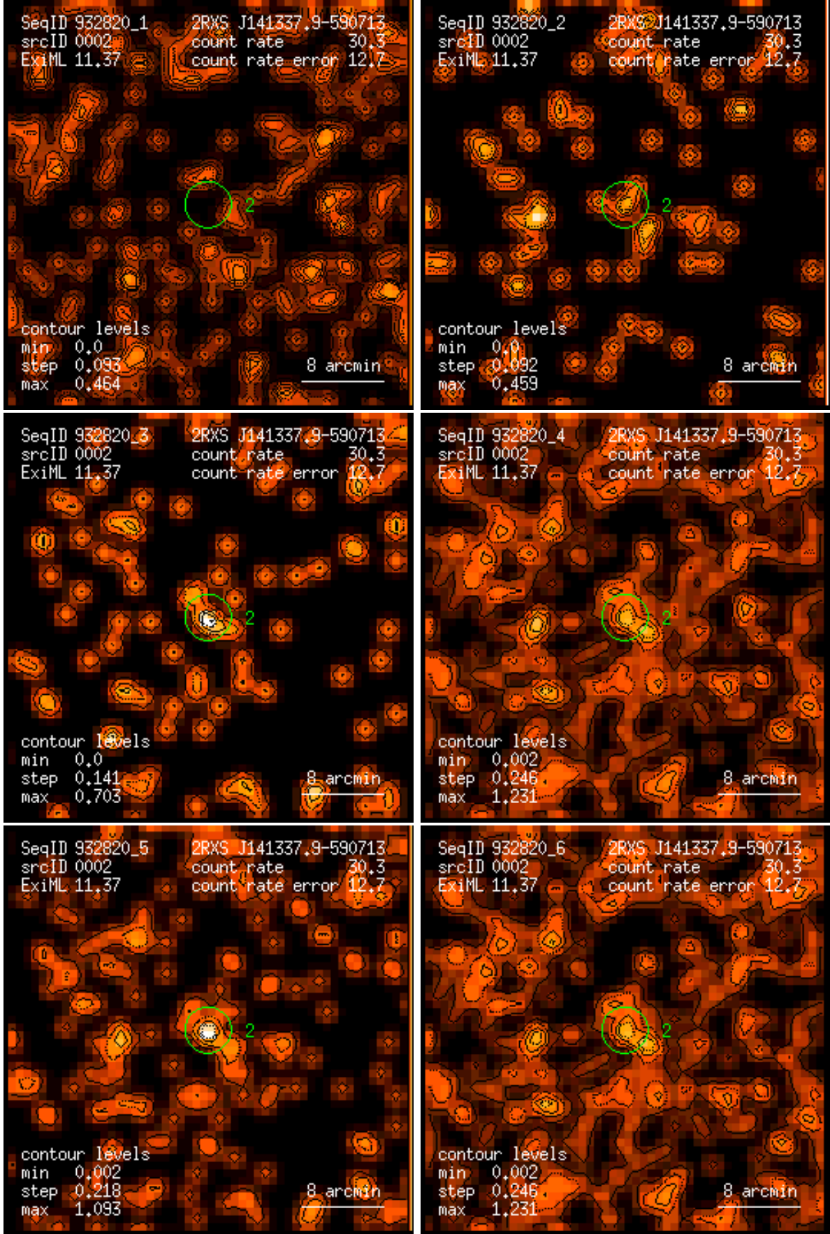
Figure 2: RASS 932820: detection 0002: band rate images, Gaussian filter: (1) PSPC channels 11 – 41, (2) 52 – 90, (3) 91 – 201, (4) 11 – 235, (5) 52 – 201, (6) 11 – 201. Broad band rates in counts/ks. Band rate contour levels in counts/ks/arcmin 2 .
