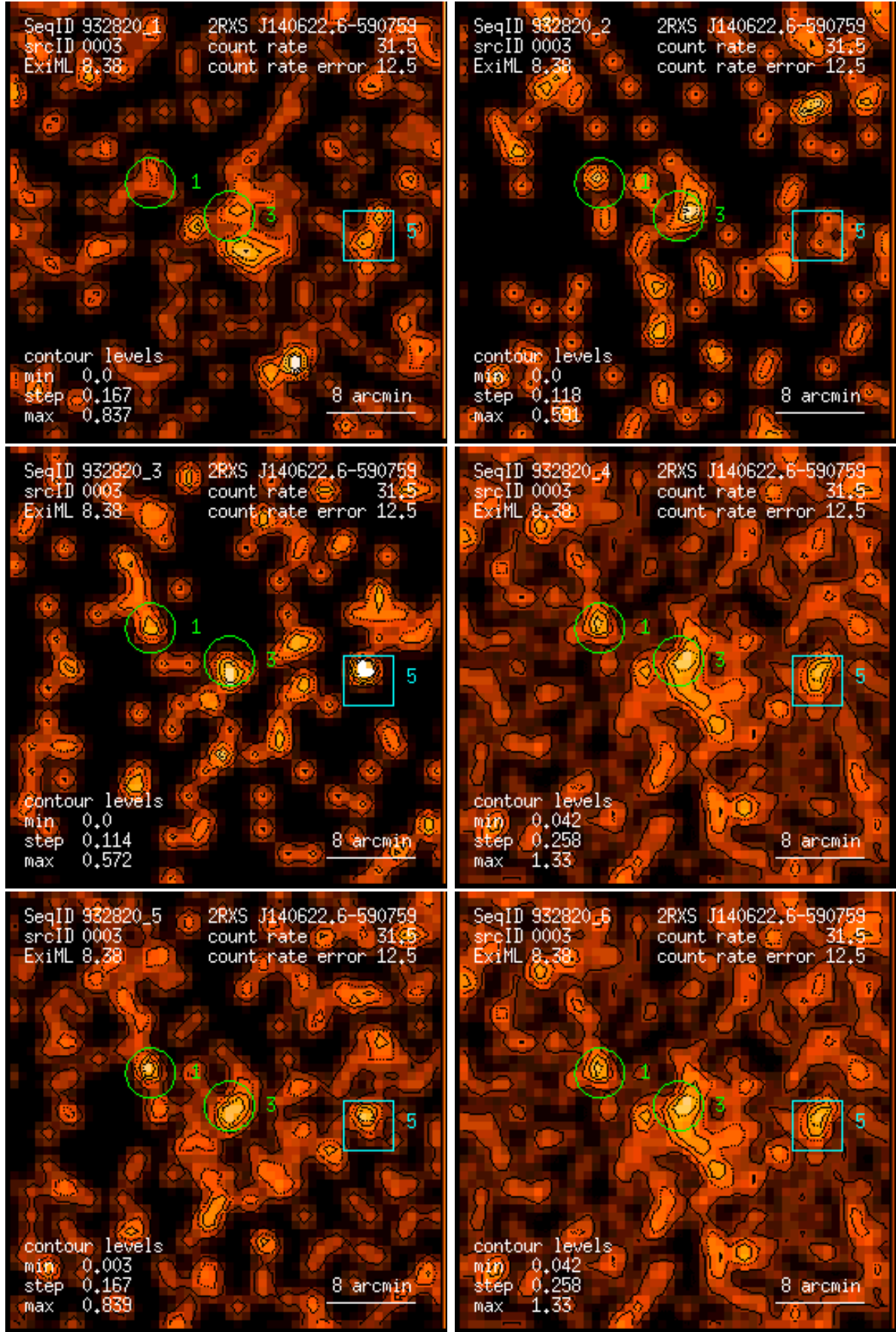
Figure 3: RASS 932820: detection 0003: band rate images, Gaussian filter: (1) PSPC channels 11 – 41, (2) 52 – 90, (3) 91 – 201, (4) 11 – 235, (5) 52 – 201, (6) 11 – 201. Broad band rates in counts/ks. Band rate contour levels in counts/ks/arcmin 2 .
