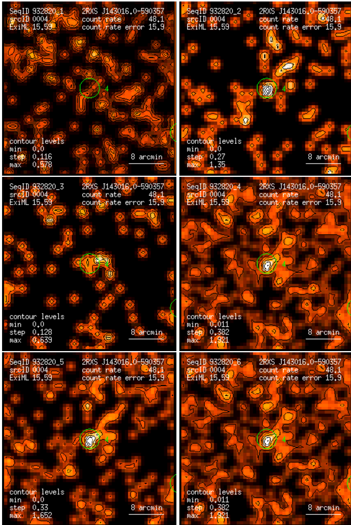
Figure 4: RASS 932820: detection 0004: band rate images, Gaussian filter: (1) PSPC channels 11 – 41, (2) 52 – 90, (3) 91 – 201, (4) 11 – 235, (5) 52 – 201, (6) 11 – 201. Broad band rates in counts/ks. Band rate contour levels in counts/ks/arcmin 2 .
