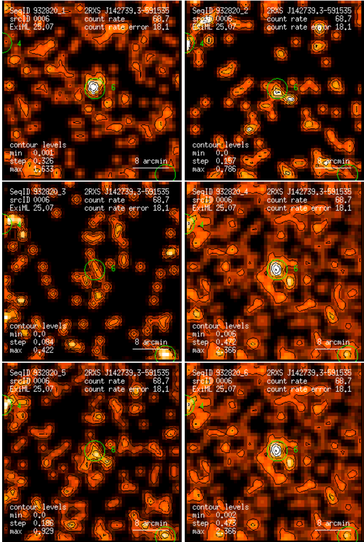
Figure 6: RASS 932820: detection 0006: band rate images, Gaussian filter: (1) PSPC channels 11 – 41, (2) 52 – 90, (3) 91 – 201, (4) 11 – 235, (5) 52 – 201, (6) 11 – 201. Broad band rates in counts/ks. Band rate contour levels in counts/ks/arcmin 2 .
