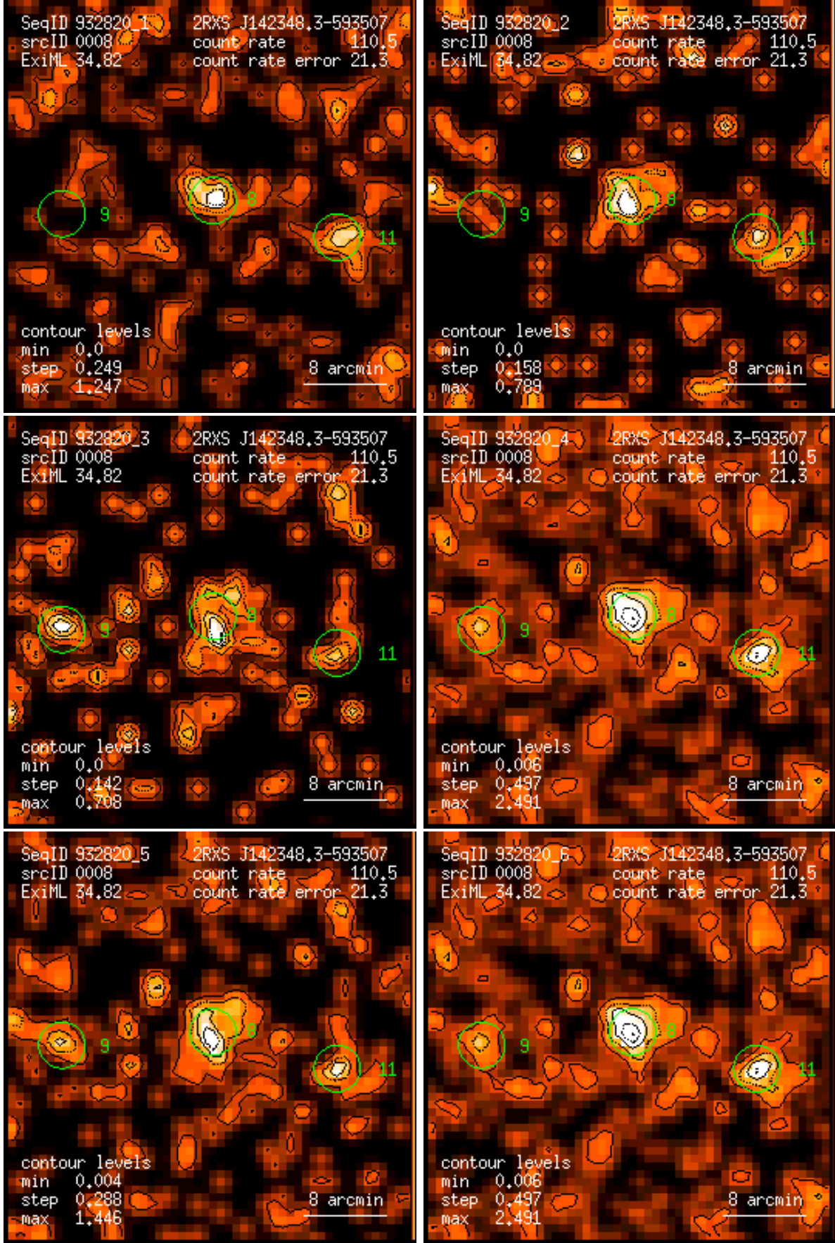
Figure 8: RASS 932820: detection 0008: band rate images, Gaussian filter: (1) PSPC channels 11 – 41, (2) 52 – 90, (3) 91 – 201, (4) 11 – 235, (5) 52 – 201, (6) 11 – 201. Broad band rates in counts/ks. Band rate contour levels in counts/ks/arcmin 2 .
