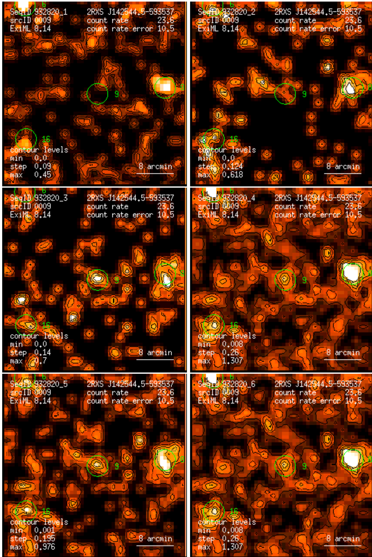
Figure 9: RASS 932820: detection 0009: band rate images, Gaussian filter: (1) PSPC channels 11 – 41, (2) 52 – 90, (3) 91 – 201, (4) 11 – 235, (5) 52 – 201, (6) 11 – 201. Broad band rates in counts/ks. Band rate contour levels in counts/ks/arcmin 2 .
