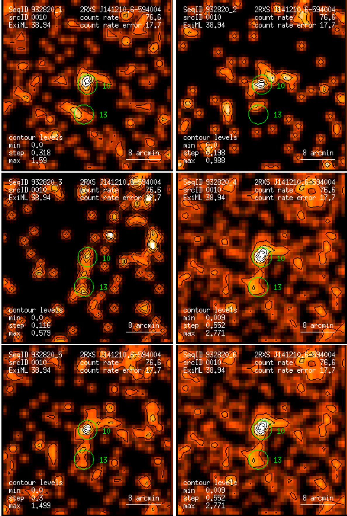
Figure 10: RASS 932820: detection 0010: band rate images, Gaussian filter: (1) PSPC channels 11 – 41, (2) 52 – 90, (3) 91 – 201, (4) 11 – 235, (5) 52 – 201, (6) 11 – 201. Broad band rates in counts/ks. Band rate contour levels in counts/ks/arcmin 2 .
