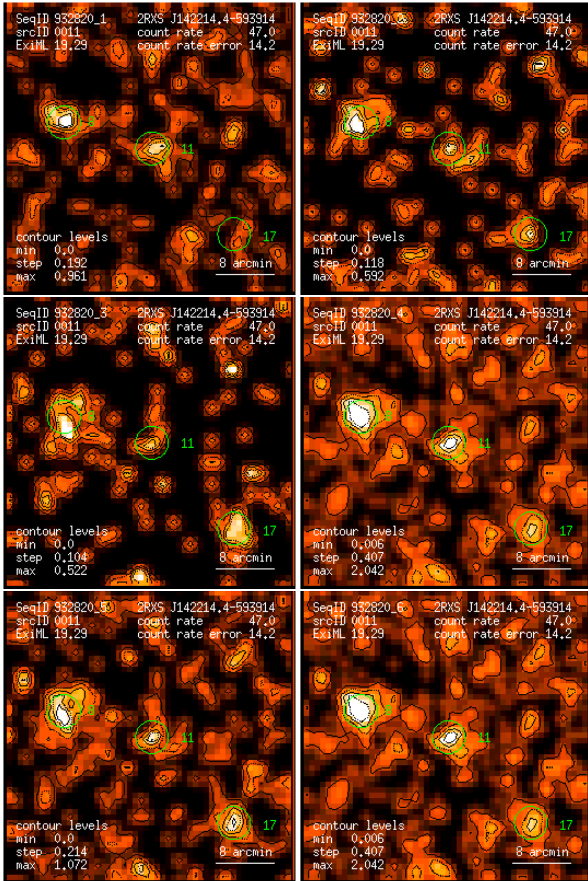
Figure 11: RASS 932820: detection 0011: band rate images, Gaussian filter: (1) PSPC channels 11 – 41, (2) 52 – 90, (3) 91 – 201, (4) 11 – 235, (5) 52 – 201, (6) 11 – 201. Broad band rates in counts/ks. Band rate contour levels in counts/ks/arcmin 2 .
