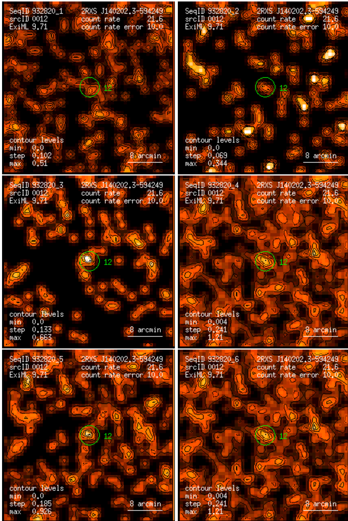
Figure 12: RASS 932820: detection 0012: band rate images, Gaussian filter: (1) PSPC channels 11 – 41, (2) 52 – 90, (3) 91 – 201, (4) 11 – 235, (5) 52 – 201, (6) 11 – 201. Broad band rates in counts/ks. Band rate contour levels in counts/ks/arcmin 2 .
