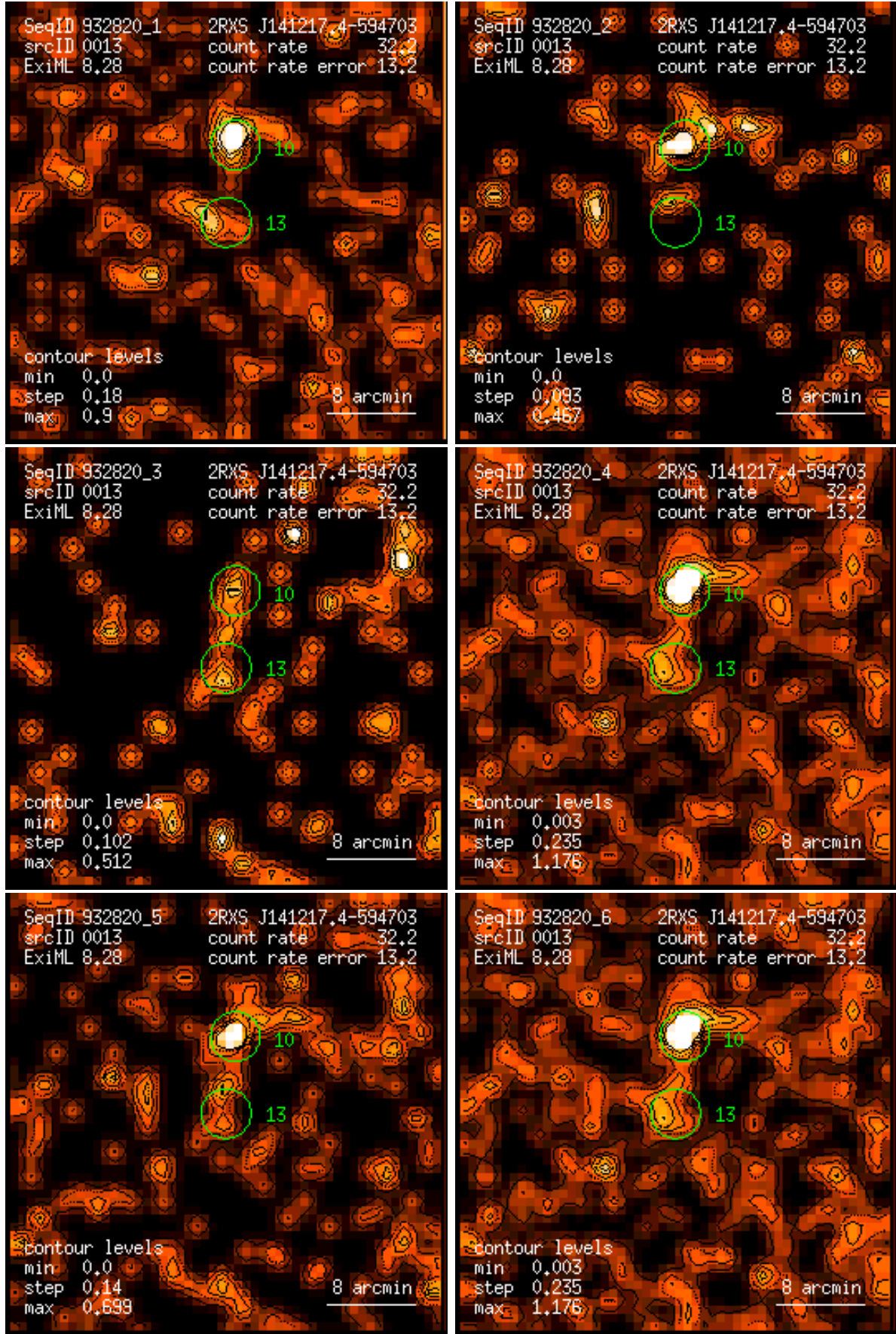
Figure 13: RASS 932820: detection 0013: band rate images, Gaussian filter: (1) PSPC channels 11 – 41, (2) 52 – 90, (3) 91 – 201, (4) 11 – 235, (5) 52 – 201, (6) 11 – 201. Broad band rates in counts/ks. Band rate contour levels in counts/ks/arcmin 2 .
