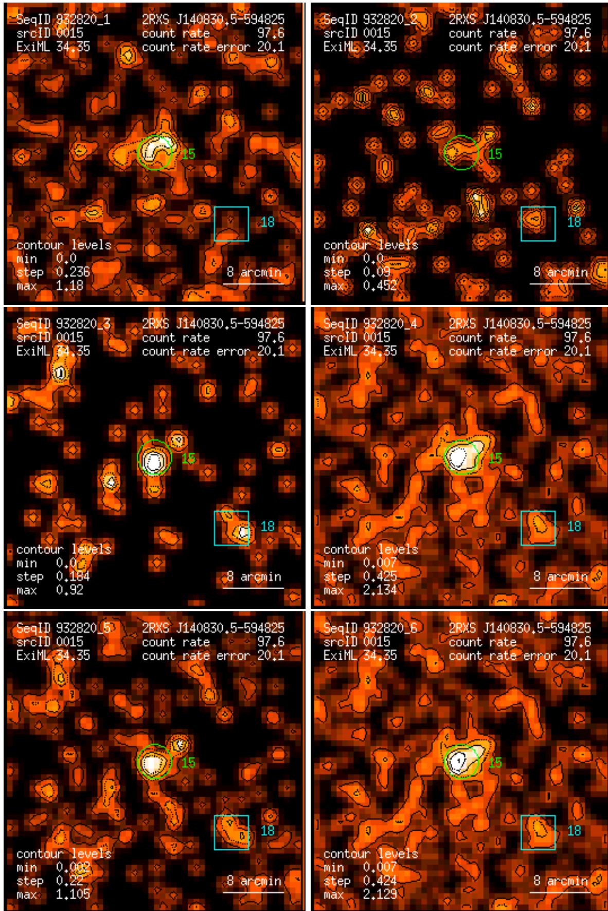
Figure 15: RASS 932820: detection 0015: band rate images, Gaussian filter: (1) PSPC channels 11 – 41, (2) 52 – 90, (3) 91 – 201, (4) 11 – 235, (5) 52 – 201, (6) 11 – 201. Broad band rates in counts/ks. Band rate contour levels in counts/ks/arcmin 2 .
