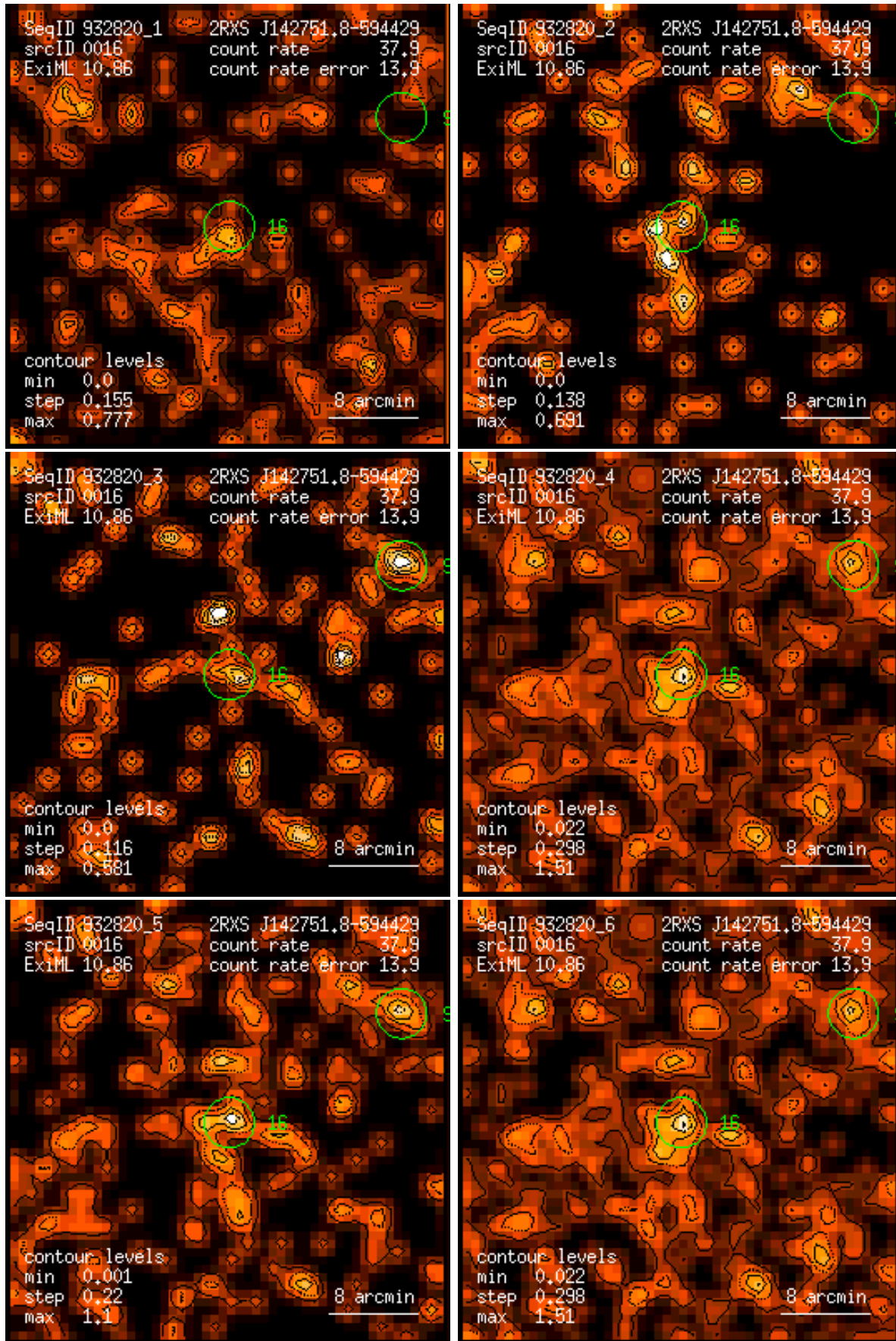
Figure 16: RASS 932820: detection 0016: band rate images, Gaussian filter: (1) PSPC channels 11 – 41, (2) 52 – 90, (3) 91 – 201, (4) 11 – 235, (5) 52 – 201, (6) 11 – 201. Broad band rates in counts/ks. Band rate contour levels in counts/ks/arcmin 2 .
