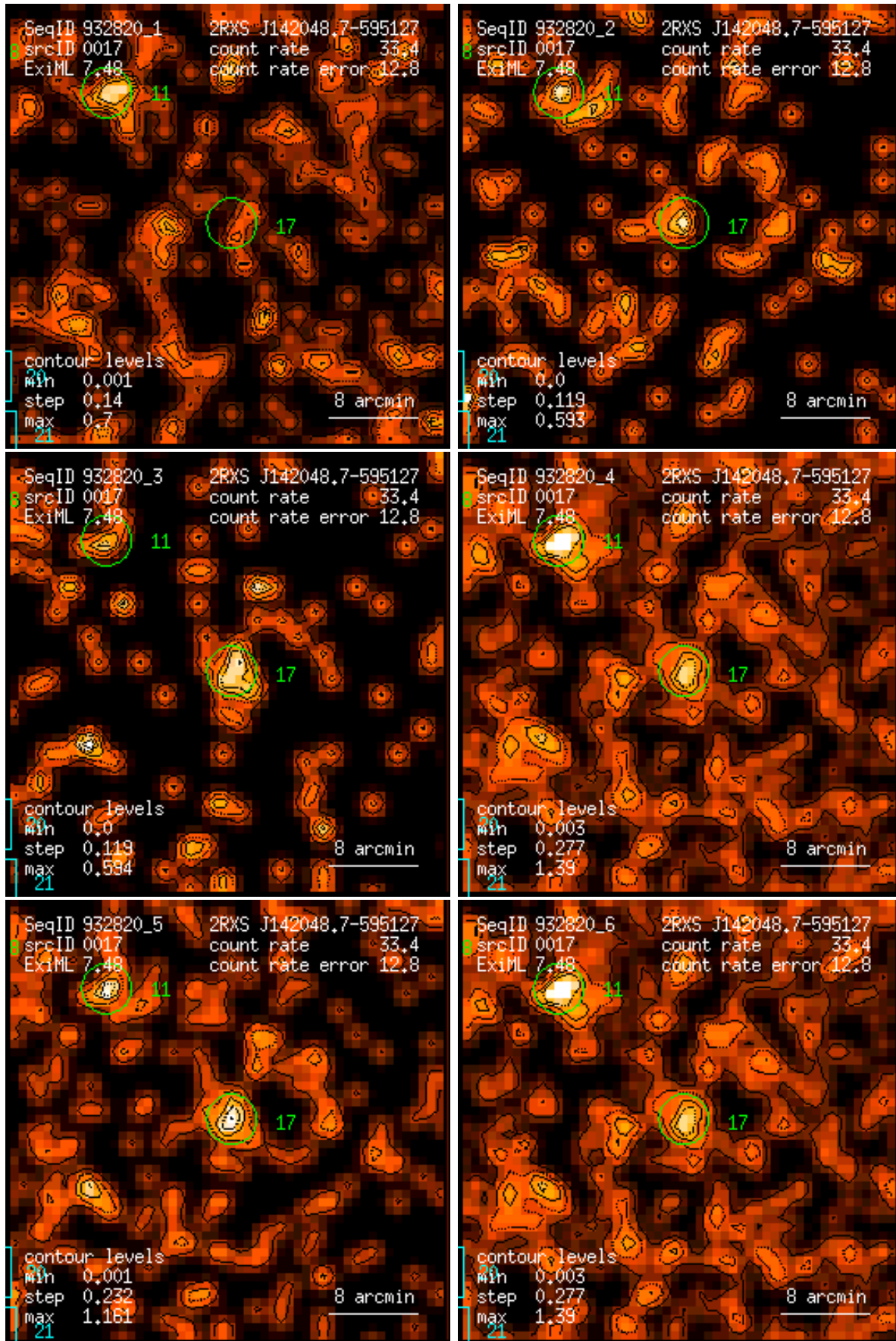
Figure 17: RASS 932820: detection 0017: band rate images, Gaussian filter: (1) PSPC channels 11 – 41, (2) 52 – 90, (3) 91 – 201, (4) 11 – 235, (5) 52 – 201, (6) 11 – 201. Broad band rates in counts/ks. Band rate contour levels in counts/ks/arcmin 2 .
