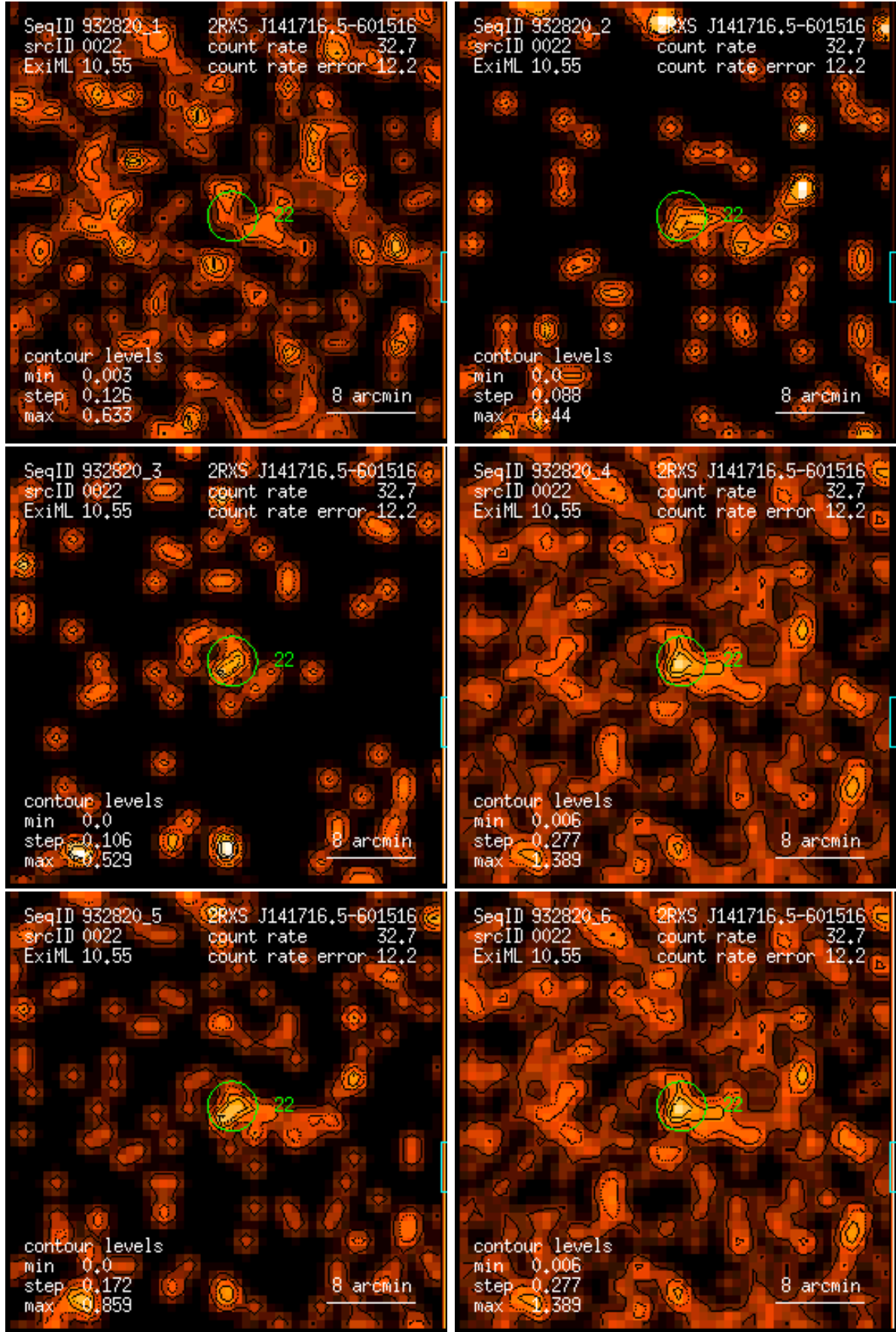
Figure 22: RASS 932820: detection 0022: band rate images, Gaussian filter: (1) PSPC channels 11 – 41, (2) 52 – 90, (3) 91 – 201, (4) 11 – 235, (5) 52 – 201, (6) 11 – 201. Broad band rates in counts/ks. Band rate contour levels in counts/ks/arcmin 2 .
