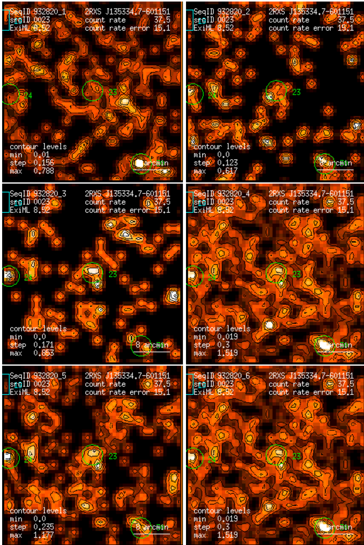
Figure 23: RASS 932820: detection 0023: band rate images, Gaussian filter: (1) PSPC channels 11 – 41, (2) 52 – 90, (3) 91 – 201, (4) 11 – 235, (5) 52 – 201, (6) 11 – 201. Broad band rates in counts/ks. Band rate contour levels in counts/ks/arcmin 2 .
