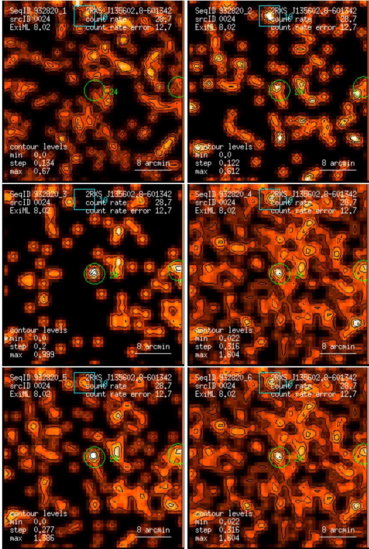
Figure 24: RASS 932820: detection 0024: band rate images, Gaussian filter: (1) PSPC channels 11 – 41, (2) 52 – 90, (3) 91 – 201, (4) 11 – 235, (5) 52 – 201, (6) 11 – 201. Broad band rates in counts/ks. Band rate contour levels in counts/ks/arcmin 2 .
