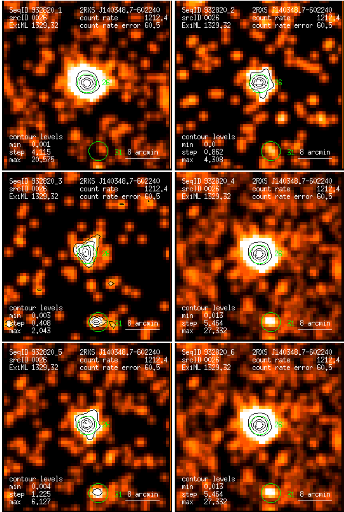
Figure 26: RASS 932820: detection 0026: band rate images, Gaussian filter: (1) PSPC channels 11 – 41, (2) 52 – 90, (3) 91 – 201, (4) 11 – 235, (5) 52 – 201, (6) 11 – 201. Broad band rates in counts/ks. Band rate contour levels in counts/ks/arcmin 2 .
