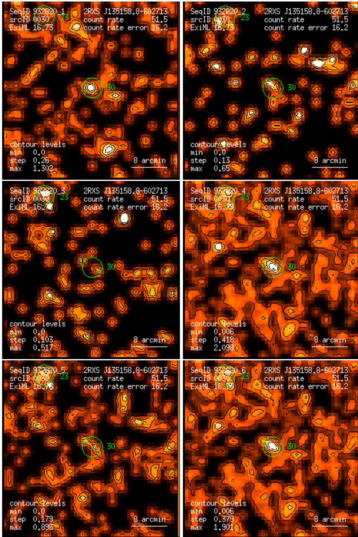
Figure 30: RASS 932820: detection 0030: band rate images, Gaussian filter: (1) PSPC channels 11 – 41, (2) 52 – 90, (3) 91 – 201, (4) 11 – 235, (5) 52 – 201, (6) 11 – 201. Broad band rates in counts/ks. Band rate contour levels in counts/ks/arcmin 2 .
