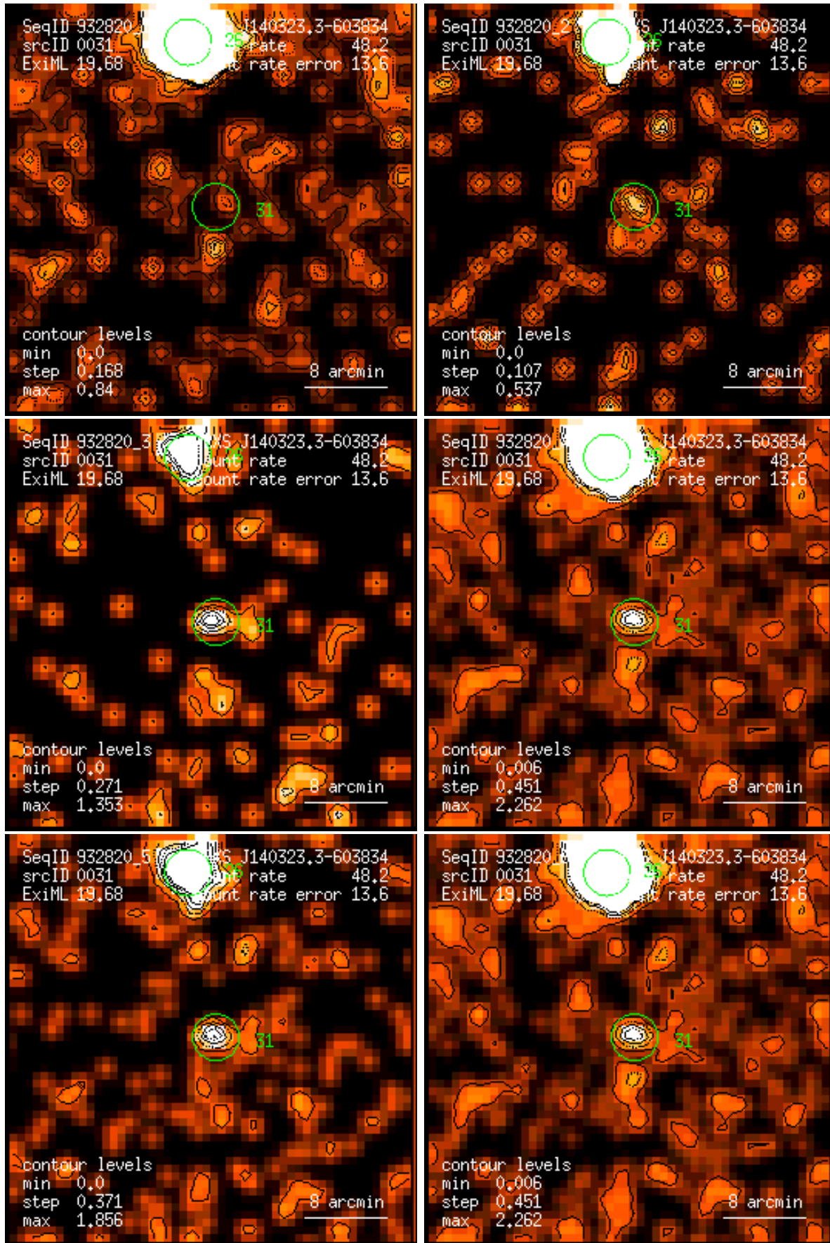
Figure 31: RASS 932820: detection 0031: band rate images, Gaussian filter: (1) PSPC channels 11 – 41, (2) 52 – 90, (3) 91 – 201, (4) 11 – 235, (5) 52 – 201, (6) 11 – 201. Broad band rates in counts/ks. Band rate contour levels in counts/ks/arcmin 2 .
