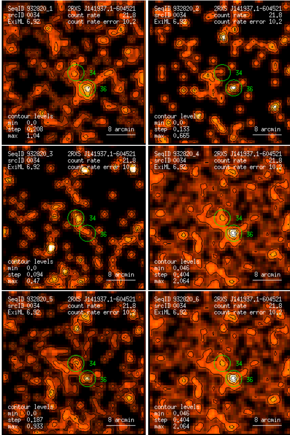
Figure 34: RASS 932820: detection 0034: band rate images, Gaussian filter: (1) PSPC channels 11 – 41, (2) 52 – 90, (3) 91 – 201, (4) 11 – 235, (5) 52 – 201, (6) 11 – 201. Broad band rates in counts/ks. Band rate contour levels in counts/ks/arcmin 2 .
