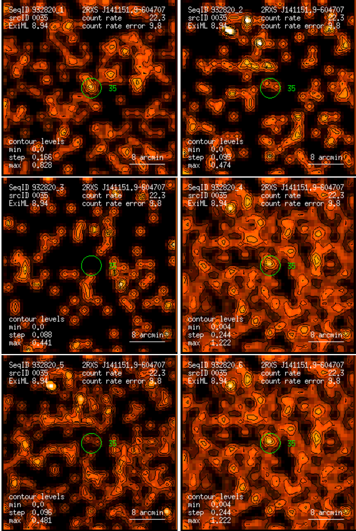
Figure 35: RASS 932820: detection 0035: band rate images, Gaussian filter: (1) PSPC channels 11 – 41, (2) 52 – 90, (3) 91 – 201, (4) 11 – 235, (5) 52 – 201, (6) 11 – 201. Broad band rates in counts/ks. Band rate contour levels in counts/ks/arcmin 2 .
