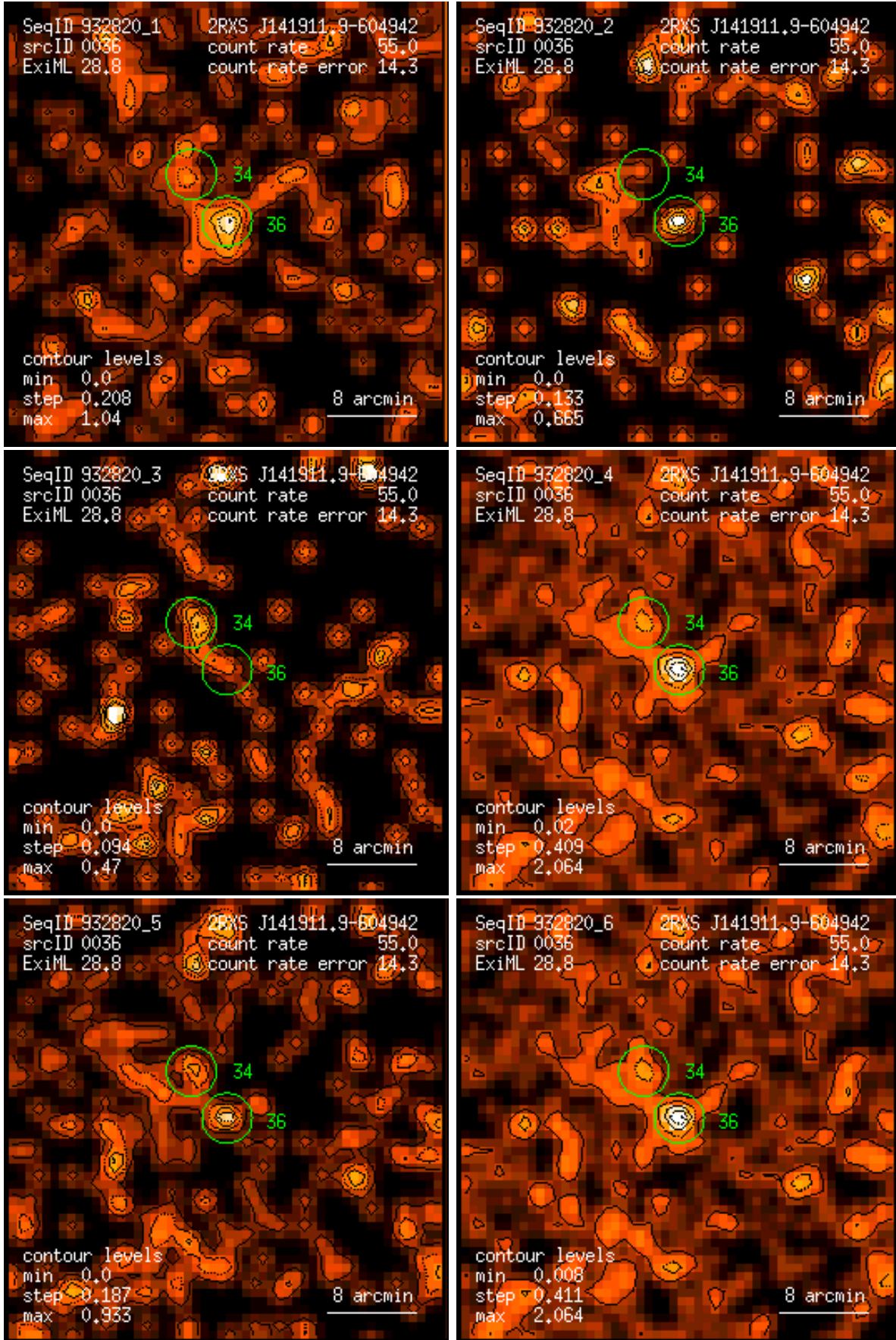
Figure 36: RASS 932820: detection 0036: band rate images, Gaussian filter: (1) PSPC channels 11 – 41, (2) 52 – 90, (3) 91 – 201, (4) 11 – 235, (5) 52 – 201, (6) 11 – 201. Broad band rates in counts/ks. Band rate contour levels in counts/ks/arcmin 2 .
