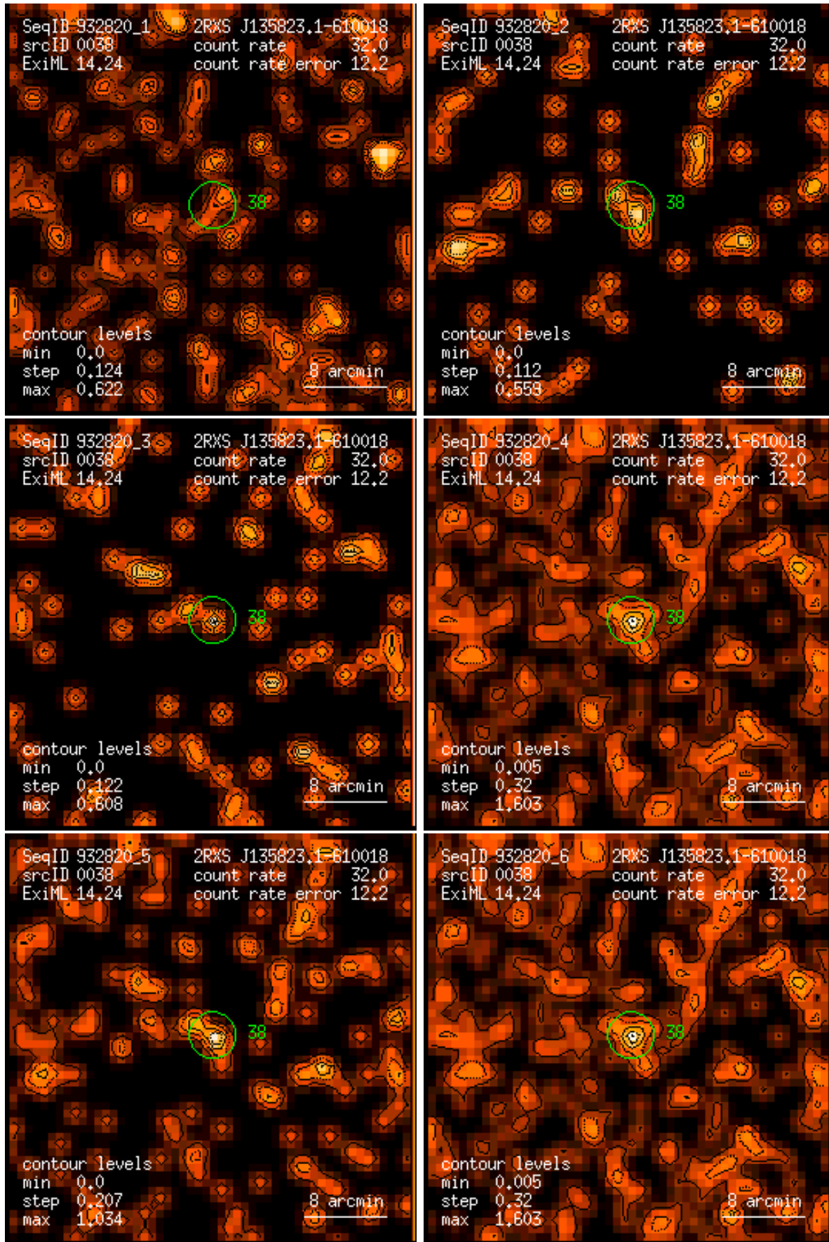
Figure 38: RASS 932820: detection 0038: band rate images, Gaussian filter: (1) PSPC channels 11 – 41, (2) 52 – 90, (3) 91 – 201, (4) 11 – 235, (5) 52 – 201, (6) 11 – 201. Broad band rates in counts/ks. Band rate contour levels in counts/ks/arcmin 2 .
