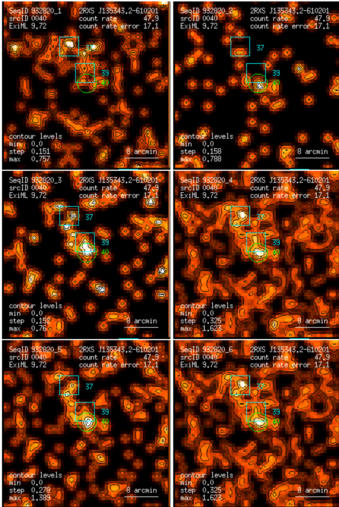
Figure 40: RASS 932820: detection 0040: band rate images, Gaussian filter: (1) PSPC channels 11 – 41, (2) 52 – 90, (3) 91 – 201, (4) 11 – 235, (5) 52 – 201, (6) 11 – 201. Broad band rates in counts/ks. Band rate contour levels in counts/ks/arcmin 2 .
