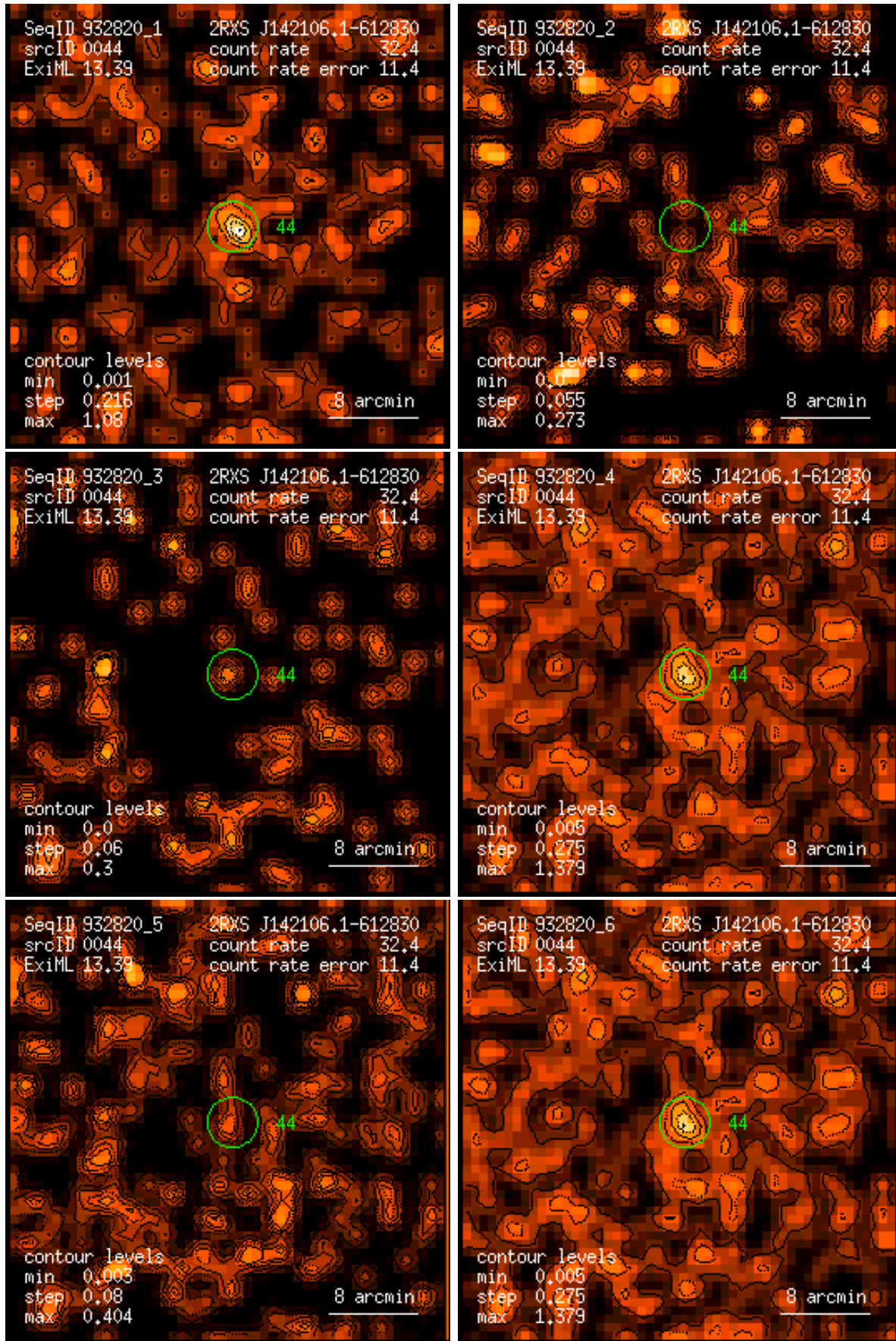
Figure 44: RASS 932820: detection 0044: band rate images, Gaussian filter: (1) PSPC channels 11 – 41, (2) 52 – 90, (3) 91 – 201, (4) 11 – 235, (5) 52 – 201, (6) 11 – 201. Broad band rates in counts/ks. Band rate contour levels in counts/ks/arcmin 2 .
