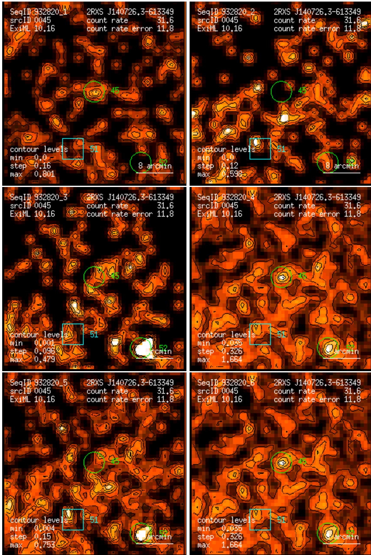
Figure 45: RASS 932820: detection 0045: band rate images, Gaussian filter: (1) PSPC channels 11 – 41, (2) 52 – 90, (3) 91 – 201, (4) 11 – 235, (5) 52 – 201, (6) 11 – 201. Broad band rates in counts/ks. Band rate contour levels in counts/ks/arcmin 2 .
