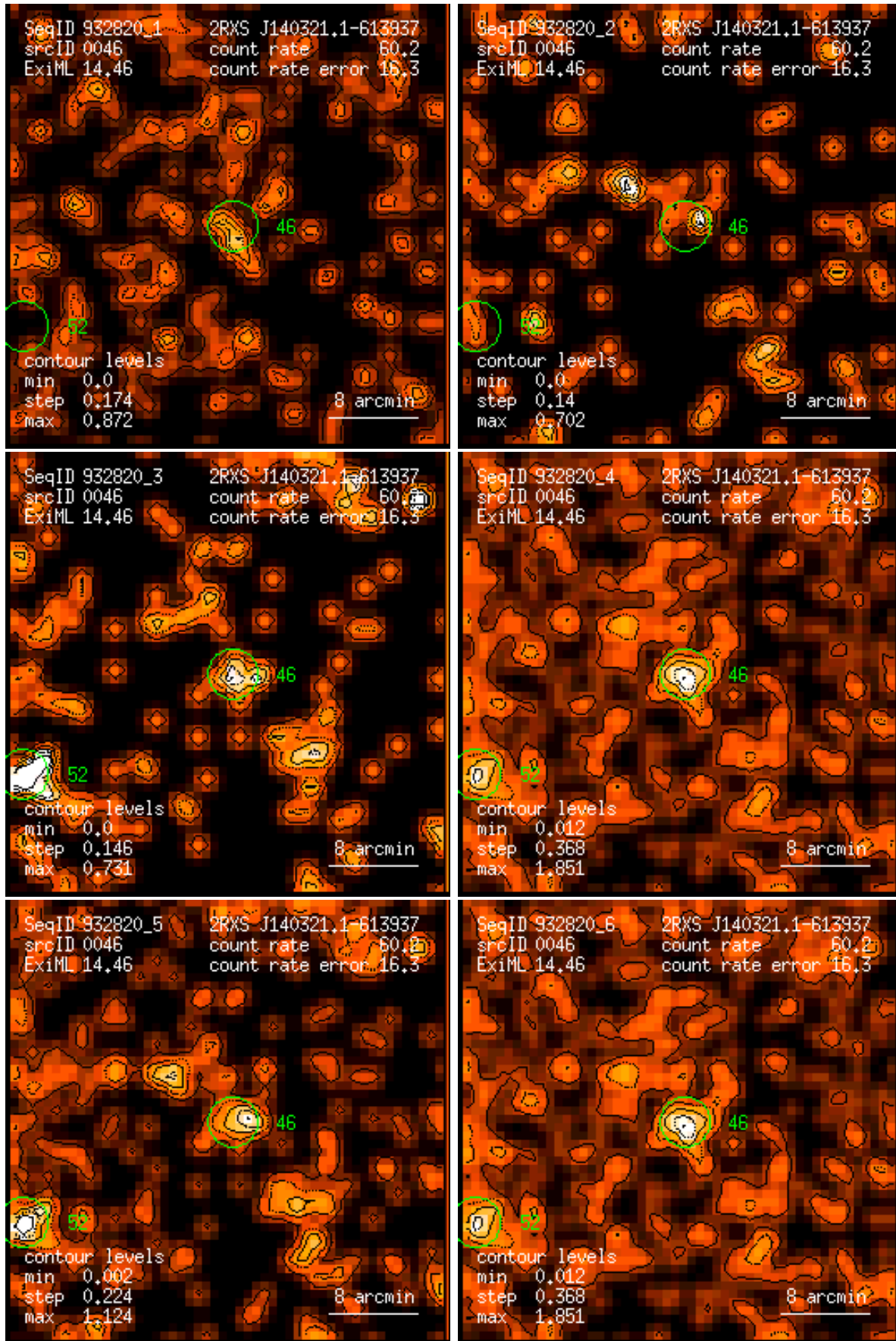
Figure 46: RASS 932820: detection 0046: band rate images, Gaussian filter: (1) PSPC channels 11 – 41, (2) 52 – 90, (3) 91 – 201, (4) 11 – 235, (5) 52 – 201, (6) 11 – 201. Broad band rates in counts/ks. Band rate contour levels in counts/ks/arcmin 2 .
