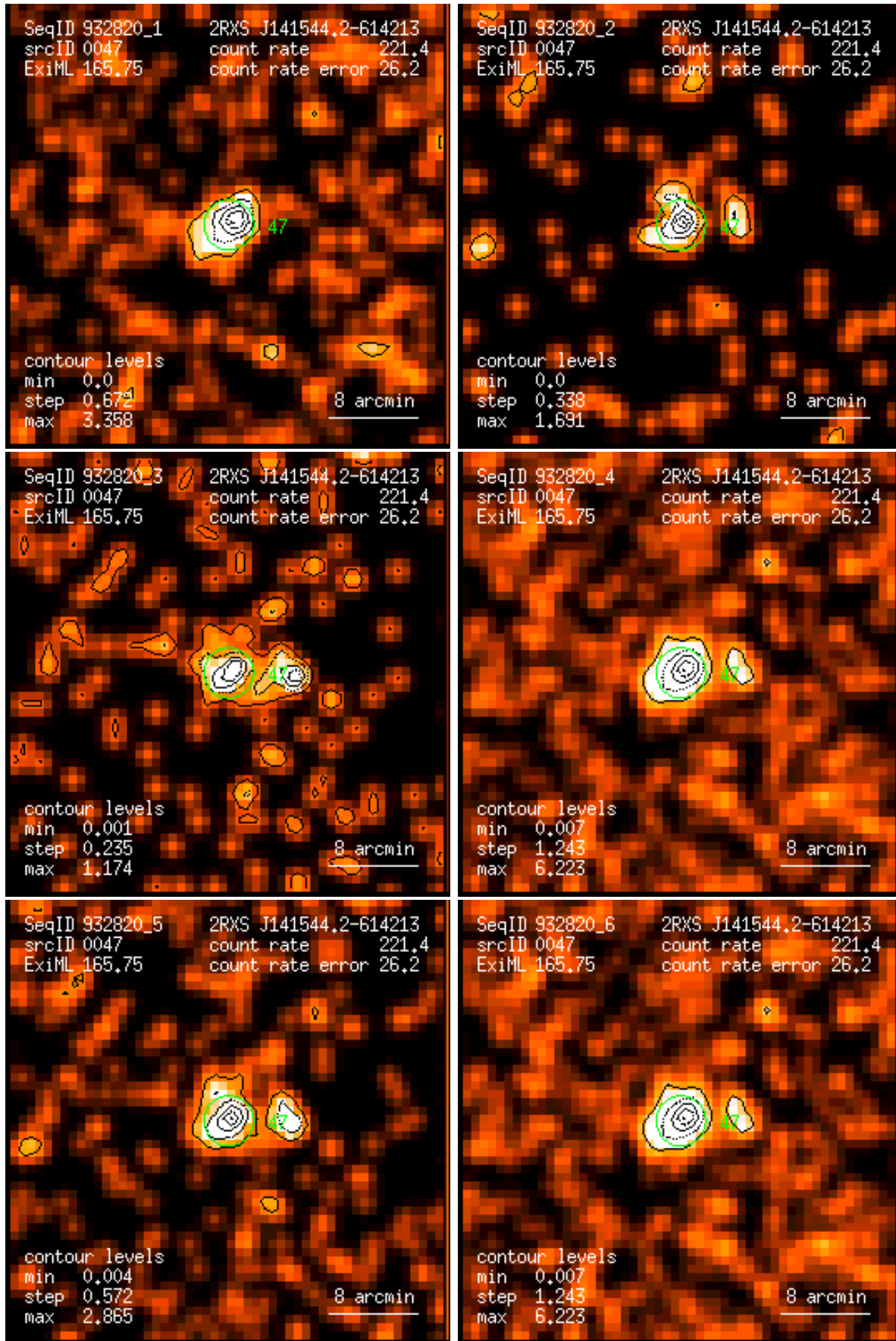
Figure 47: RASS 932820: detection 0047: band rate images, Gaussian filter: (1) PSPC channels 11 – 41, (2) 52 – 90, (3) 91 – 201, (4) 11 – 235, (5) 52 – 201, (6) 11 – 201. Broad band rates in counts/ks. Band rate contour levels in counts/ks/arcmin 2 .
