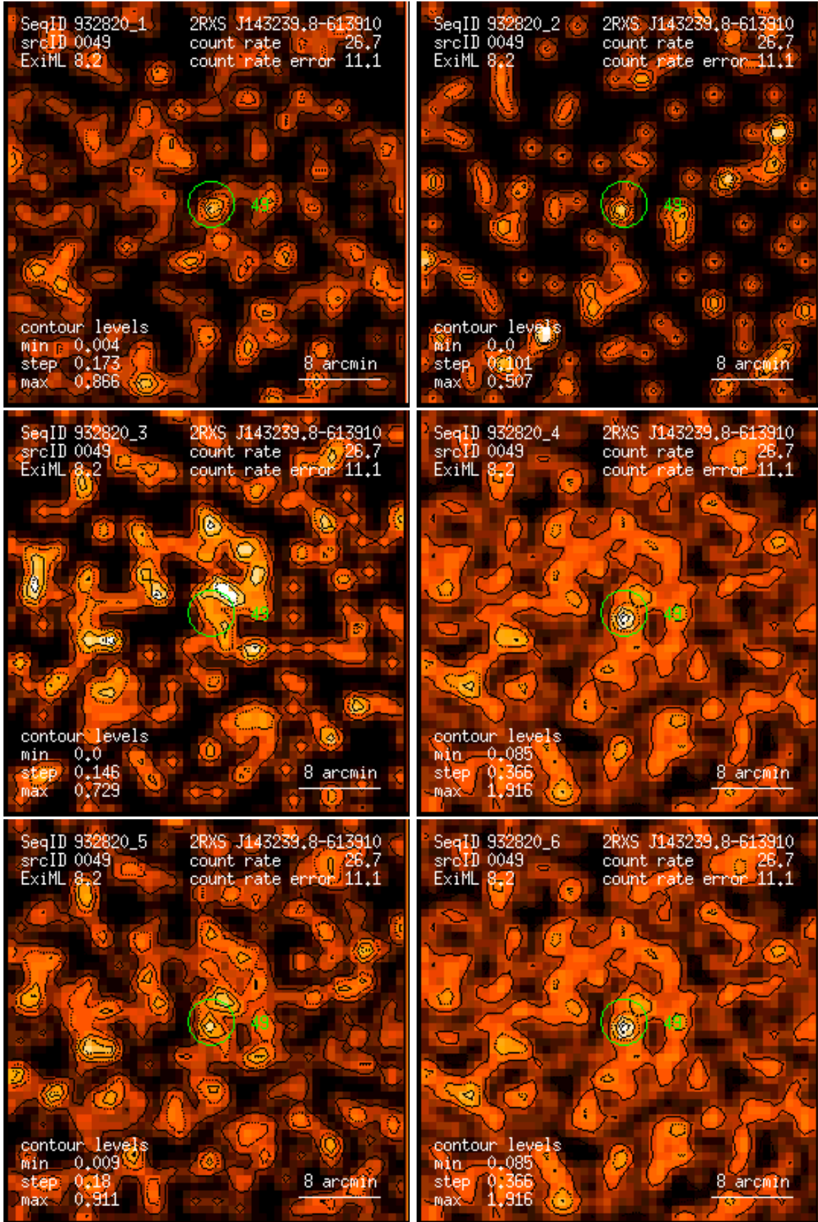
Figure 49: RASS 932820: detection 0049: band rate images, Gaussian filter: (1) PSPC channels 11 – 41, (2) 52 – 90, (3) 91 – 201, (4) 11 – 235, (5) 52 – 201, (6) 11 – 201. Broad band rates in counts/ks. Band rate contour levels in counts/ks/arcmin 2 .
