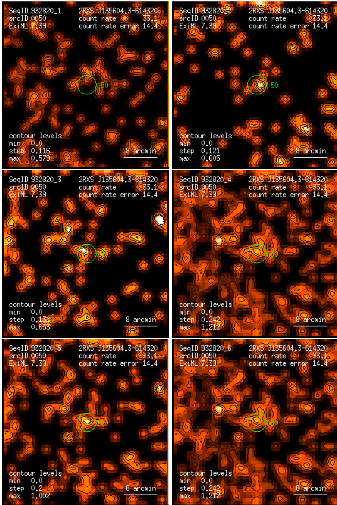
Figure 50: RASS 932820: detection 0050: band rate images, Gaussian filter: (1) PSPC channels 11 – 41, (2) 52 – 90, (3) 91 – 201, (4) 11 – 235, (5) 52 – 201, (6) 11 – 201. Broad band rates in counts/ks. Band rate contour levels in counts/ks/arcmin 2 .
