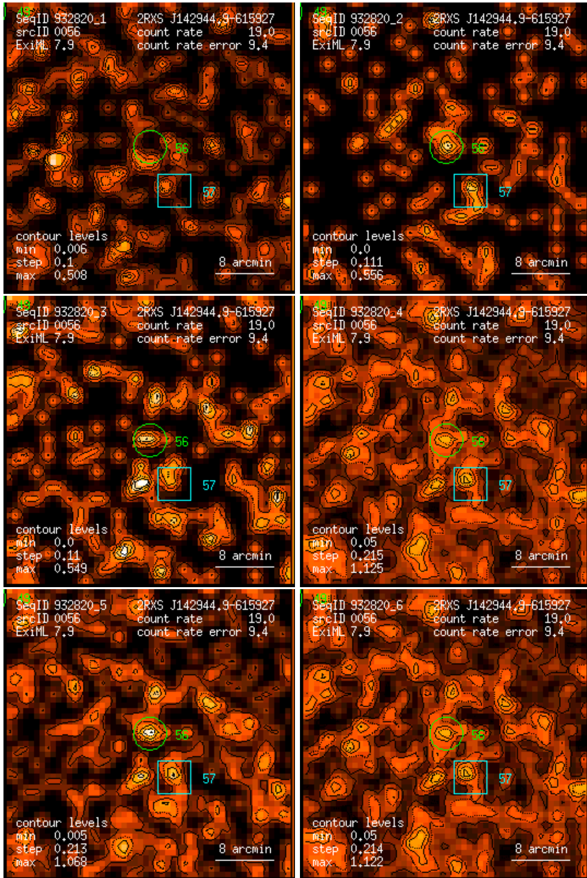
Figure 56: RASS 932820: detection 0056: band rate images, Gaussian filter: (1) PSPC channels 11 – 41, (2) 52 – 90, (3) 91 – 201, (4) 11 – 235, (5) 52 – 201, (6) 11 – 201. Broad band rates in counts/ks. Band rate contour levels in counts/ks/arcmin 2 .
