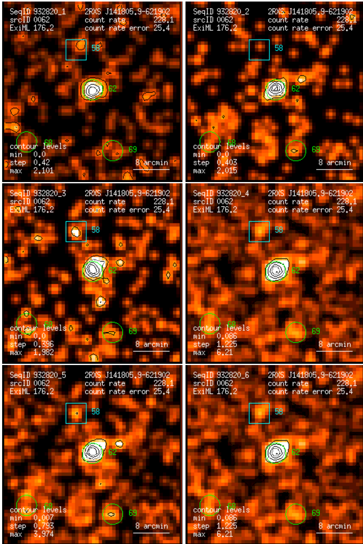
Figure 62: RASS 932820: detection 0062: band rate images, Gaussian filter: (1) PSPC channels 11 – 41, (2) 52 – 90, (3) 91 – 201, (4) 11 – 235, (5) 52 – 201, (6) 11 – 201. Broad band rates in counts/ks. Band rate contour levels in counts/ks/arcmin 2 .
