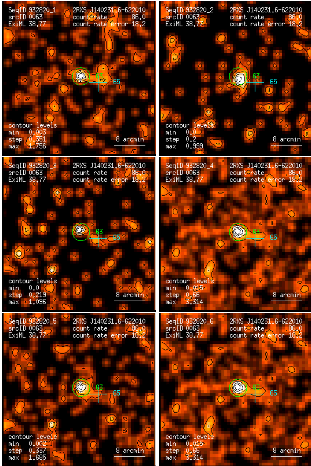
Figure 63: RASS 932820: detection 0063: band rate images, Gaussian filter: (1) PSPC channels 11 – 41, (2) 52 – 90, (3) 91 – 201, (4) 11 – 235, (5) 52 – 201, (6) 11 – 201. Broad band rates in counts/ks. Band rate contour levels in counts/ks/arcmin 2 .
