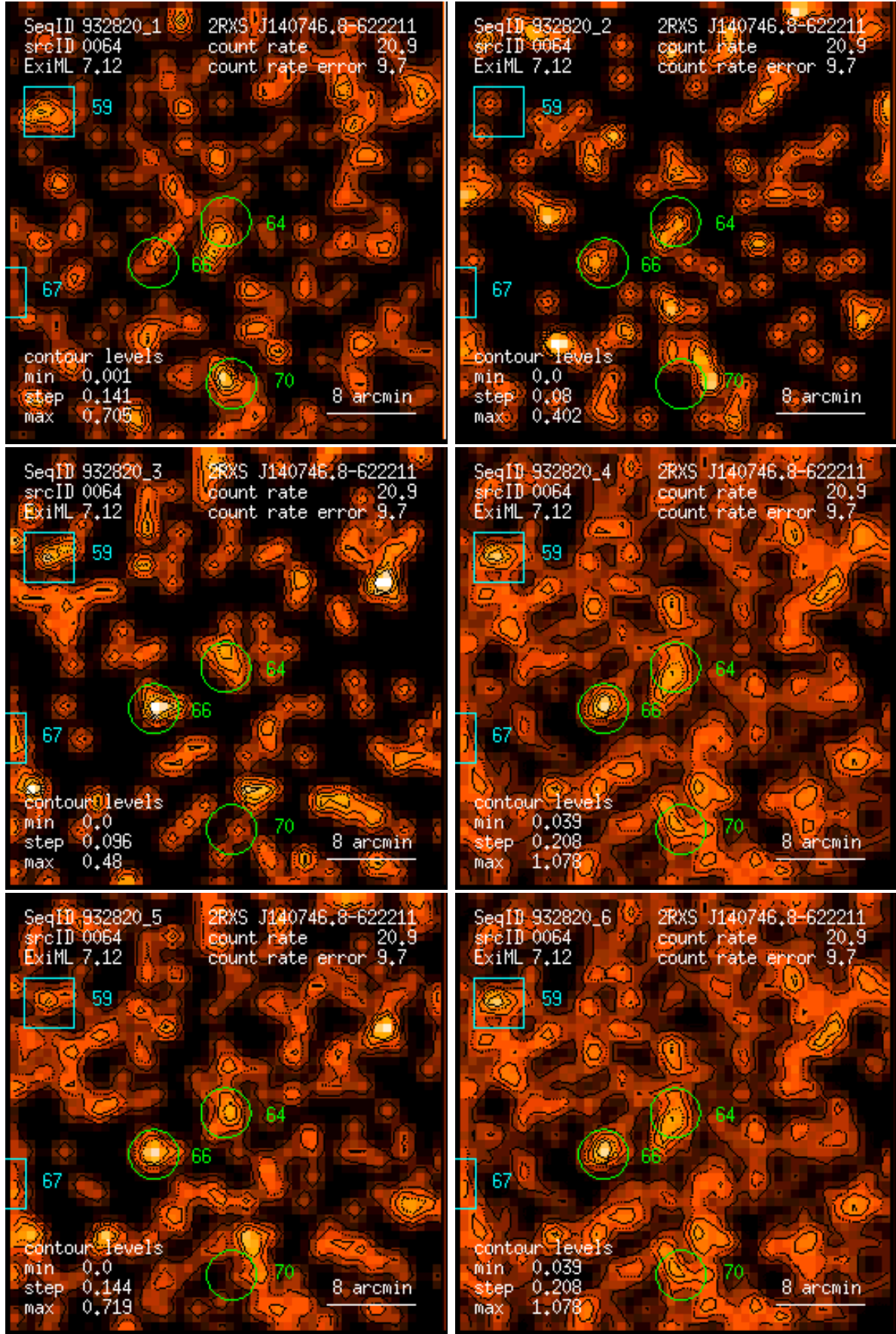
Figure 64: RASS 932820: detection 0064: band rate images, Gaussian filter: (1) PSPC channels 11 – 41, (2) 52 – 90, (3) 91 – 201, (4) 11 – 235, (5) 52 – 201, (6) 11 – 201. Broad band rates in counts/ks. Band rate contour levels in counts/ks/arcmin 2 .
