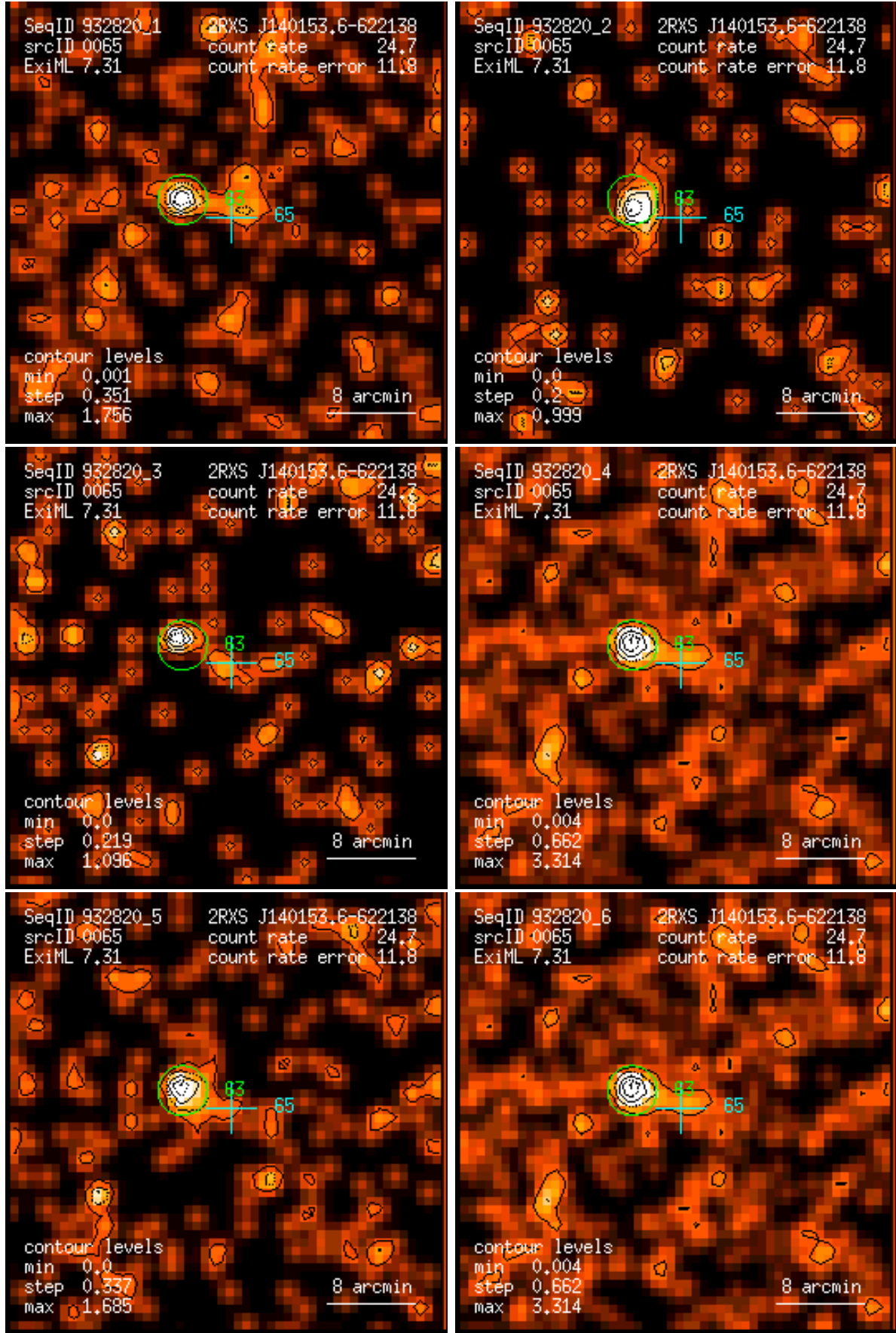
Figure 65: RASS 932820: detection 0065: band rate images, Gaussian filter: (1) PSPC channels 11 – 41, (2) 52 – 90, (3) 91 – 201, (4) 11 – 235, (5) 52 – 201, (6) 11 – 201. Broad band rates in counts/ks. Band rate contour levels in counts/ks/arcmin 2 .
