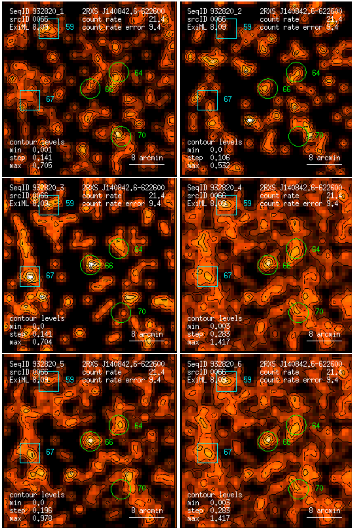
Figure 66: RASS 932820: detection 0066: band rate images, Gaussian filter: (1) PSPC channels 11 – 41, (2) 52 – 90, (3) 91 – 201, (4) 11 – 235, (5) 52 – 201, (6) 11 – 201. Broad band rates in counts/ks. Band rate contour levels in counts/ks/arcmin 2 .
