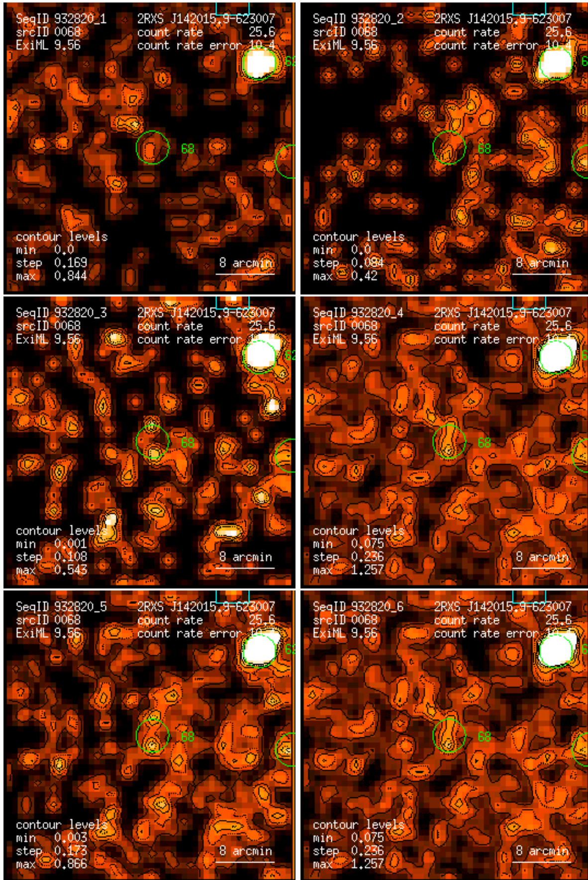
Figure 68: RASS 932820: detection 0068: band rate images, Gaussian filter: (1) PSPC channels 11 – 41, (2) 52 – 90, (3) 91 – 201, (4) 11 – 235, (5) 52 – 201, (6) 11 – 201. Broad band rates in counts/ks. Band rate contour levels in counts/ks/arcmin 2 .
