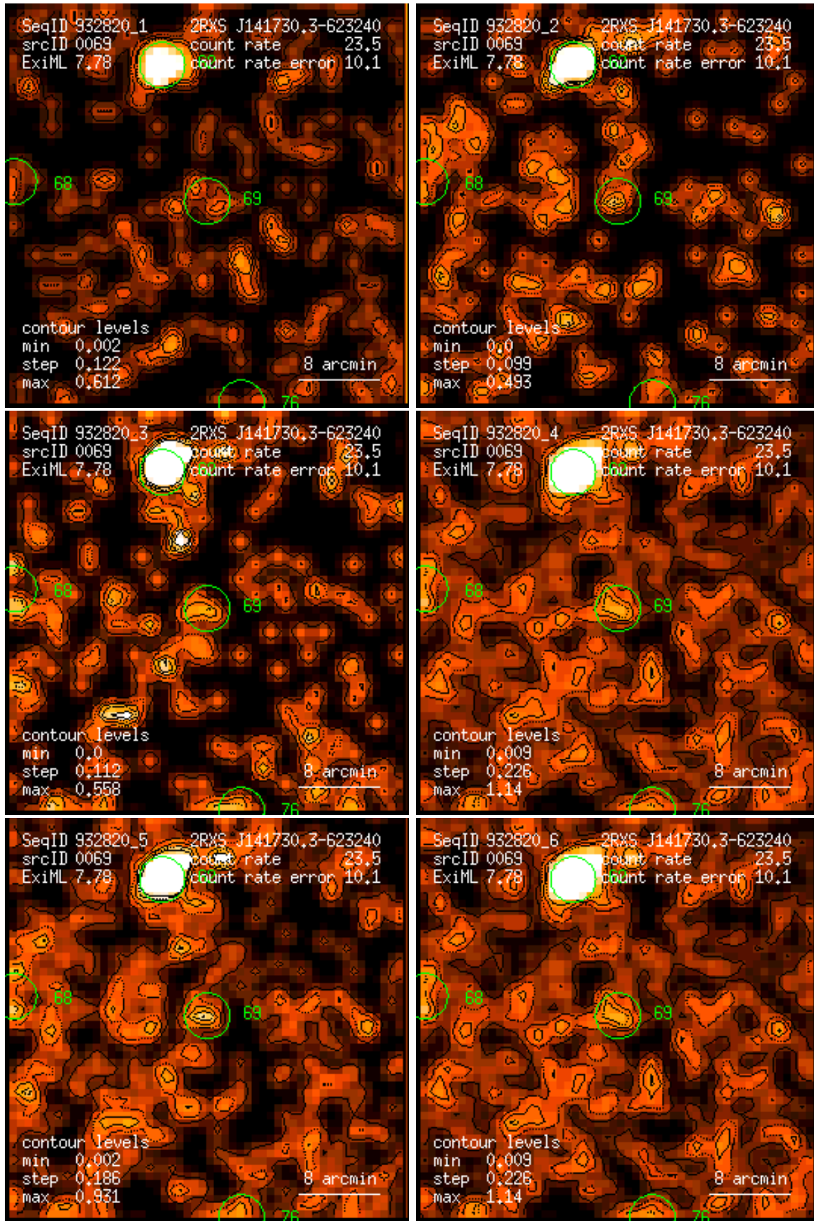
Figure 69: RASS 932820: detection 0069: band rate images, Gaussian filter: (1) PSPC channels 11 – 41, (2) 52 – 90, (3) 91 – 201, (4) 11 – 235, (5) 52 – 201, (6) 11 – 201. Broad band rates in counts/ks. Band rate contour levels in counts/ks/arcmin 2 .
