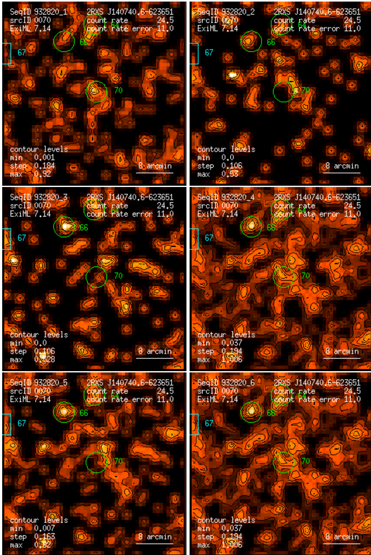
Figure 70: RASS 932820: detection 0070: band rate images, Gaussian filter: (1) PSPC channels 11 – 41, (2) 52 – 90, (3) 91 – 201, (4) 11 – 235, (5) 52 – 201, (6) 11 – 201. Broad band rates in counts/ks. Band rate contour levels in counts/ks/arcmin 2 .
