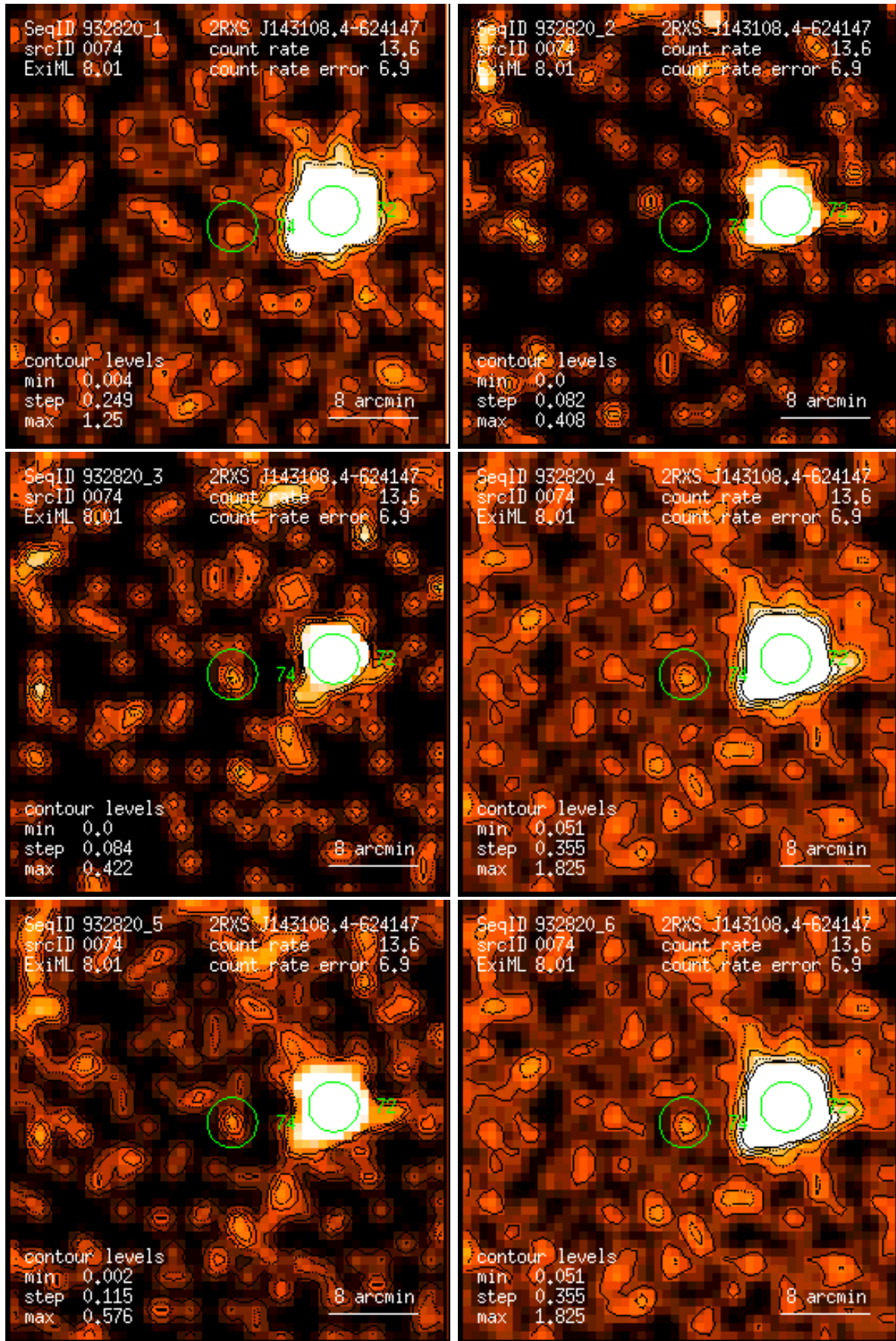
Figure 74: RASS 932820: detection 0074: band rate images, Gaussian filter: (1) PSPC channels 11 – 41, (2) 52 – 90, (3) 91 – 201, (4) 11 – 235, (5) 52 – 201, (6) 11 – 201. Broad band rates in counts/ks. Band rate contour levels in counts/ks/arcmin 2 .
