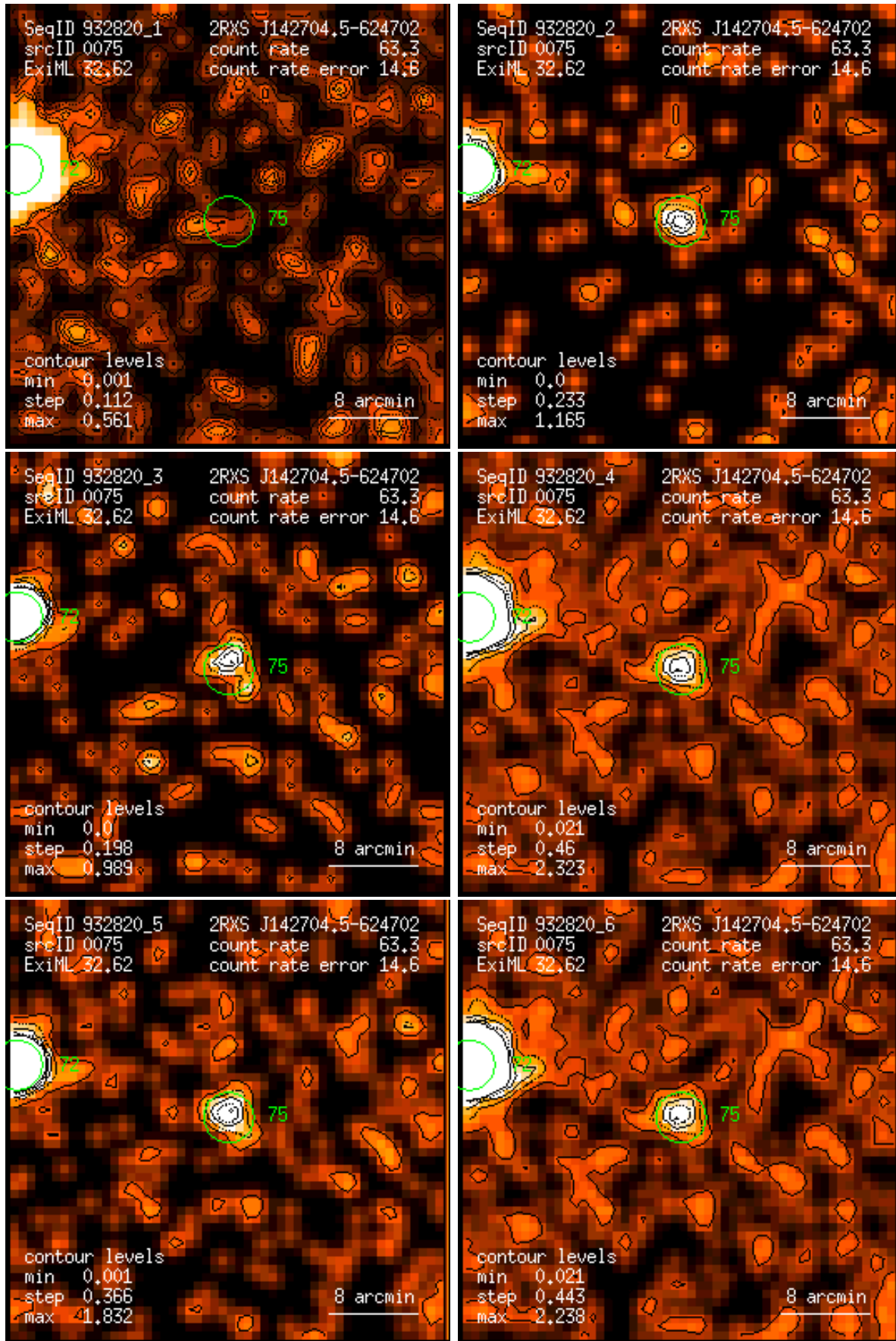
Figure 75: RASS 932820: detection 0075: band rate images, Gaussian filter: (1) PSPC channels 11 – 41, (2) 52 – 90, (3) 91 – 201, (4) 11 – 235, (5) 52 – 201, (6) 11 – 201. Broad band rates in counts/ks. Band rate contour levels in counts/ks/arcmin 2 .
