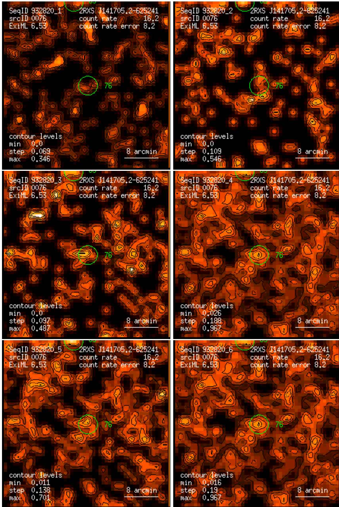
Figure 76: RASS 932820: detection 0076: band rate images, Gaussian filter: (1) PSPC channels 11 – 41, (2) 52 – 90, (3) 91 – 201, (4) 11 – 235, (5) 52 – 201, (6) 11 – 201. Broad band rates in counts/ks. Band rate contour levels in counts/ks/arcmin 2 .
