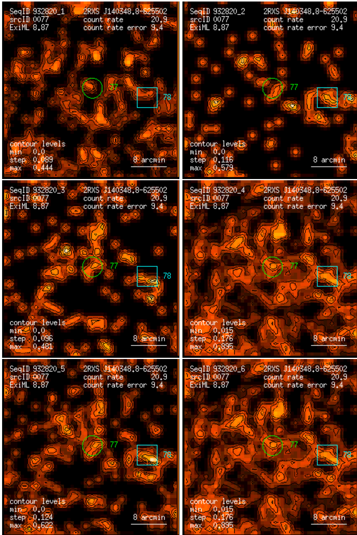
Figure 77: RASS 932820: detection 0077: band rate images, Gaussian filter: (1) PSPC channels 11 – 41, (2) 52 – 90, (3) 91 – 201, (4) 11 – 235, (5) 52 – 201, (6) 11 – 201. Broad band rates in counts/ks. Band rate contour levels in counts/ks/arcmin 2 .
