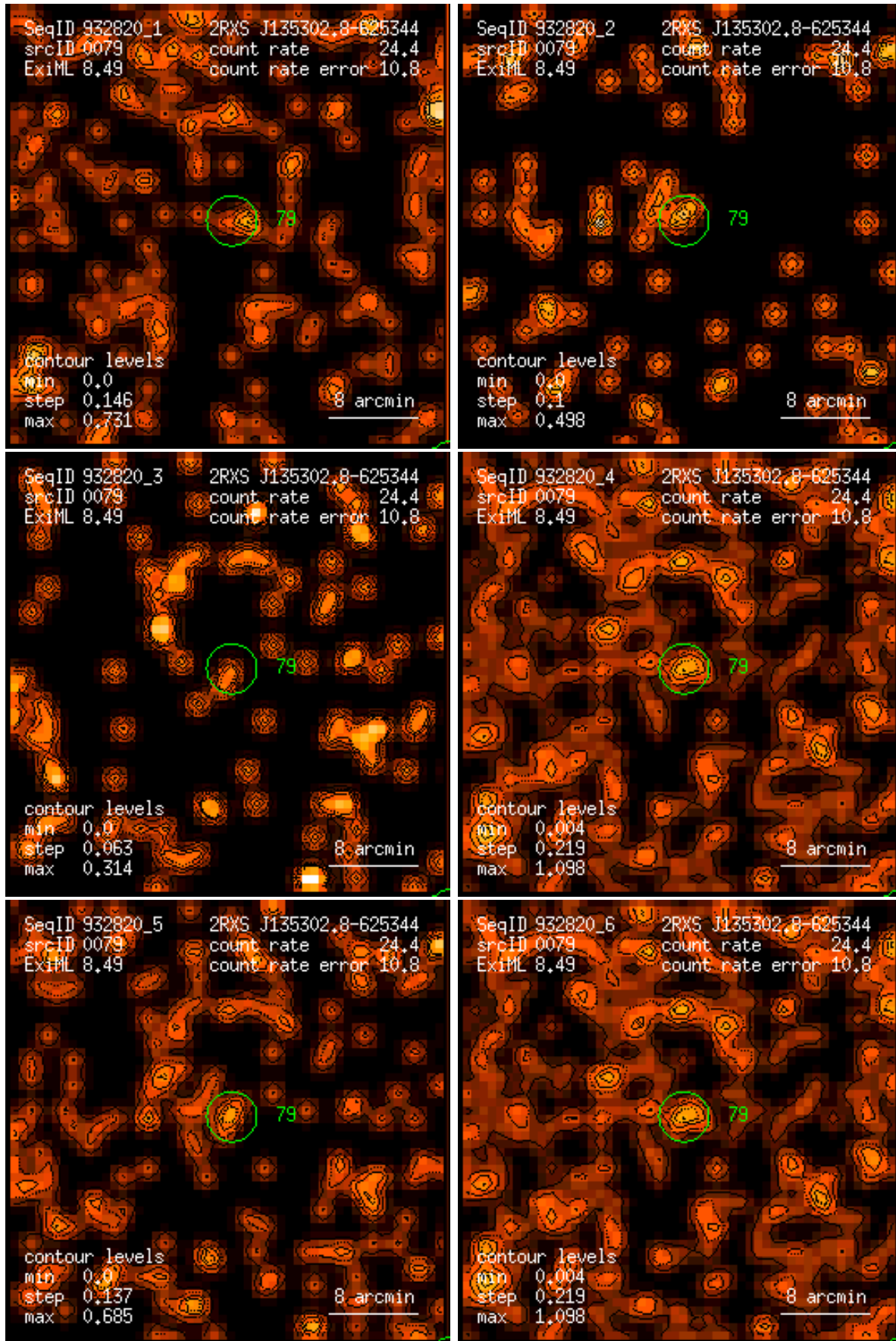
Figure 79: RASS 932820: detection 0079: band rate images, Gaussian filter: (1) PSPC channels 11 – 41, (2) 52 – 90, (3) 91 – 201, (4) 11 – 235, (5) 52 – 201, (6) 11 – 201. Broad band rates in counts/ks. Band rate contour levels in counts/ks/arcmin 2 .
