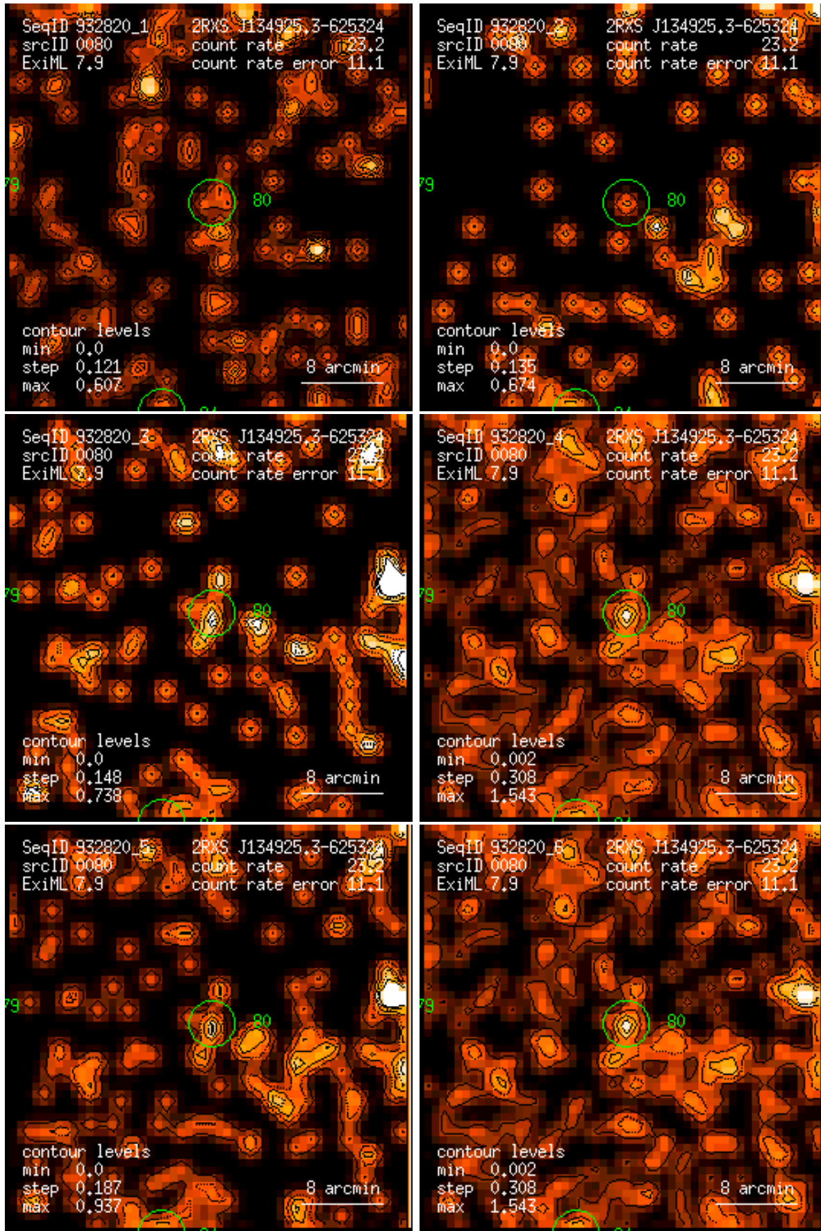
Figure 80: RASS 932820: detection 0080: band rate images, Gaussian filter: (1) PSPC channels 11 – 41, (2) 52 – 90, (3) 91 – 201, (4) 11 – 235, (5) 52 – 201, (6) 11 – 201. Broad band rates in counts/ks. Band rate contour levels in counts/ks/arcmin 2 .
