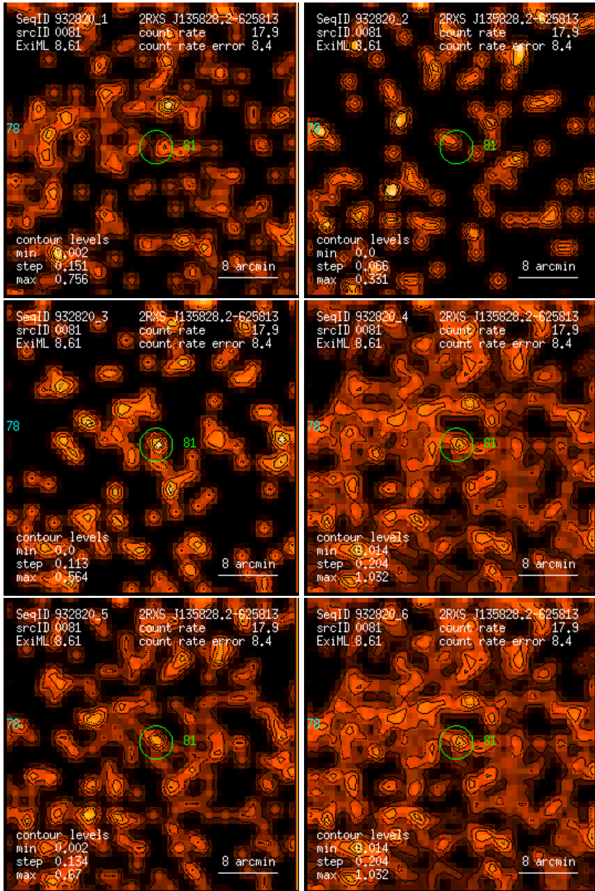
Figure 81: RASS 932820: detection 0081: band rate images, Gaussian filter: (1) PSPC channels 11 – 41, (2) 52 – 90, (3) 91 – 201, (4) 11 – 235, (5) 52 – 201, (6) 11 – 201. Broad band rates in counts/ks. Band rate contour levels in counts/ks/arcmin 2 .
