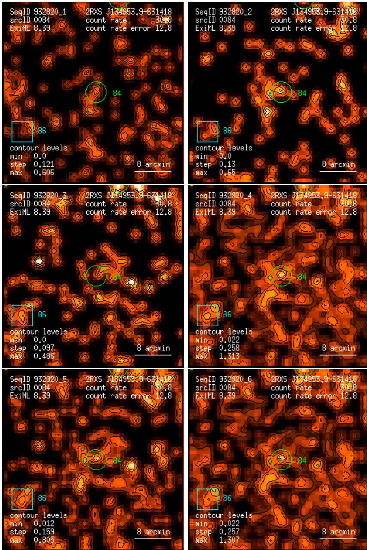
Figure 84: RASS 932820: detection 0084: band rate images, Gaussian filter: (1) PSPC channels 11 – 41, (2) 52 – 90, (3) 91 – 201, (4) 11 – 235, (5) 52 – 201, (6) 11 – 201. Broad band rates in counts/ks. Band rate contour levels in counts/ks/arcmin 2 .
