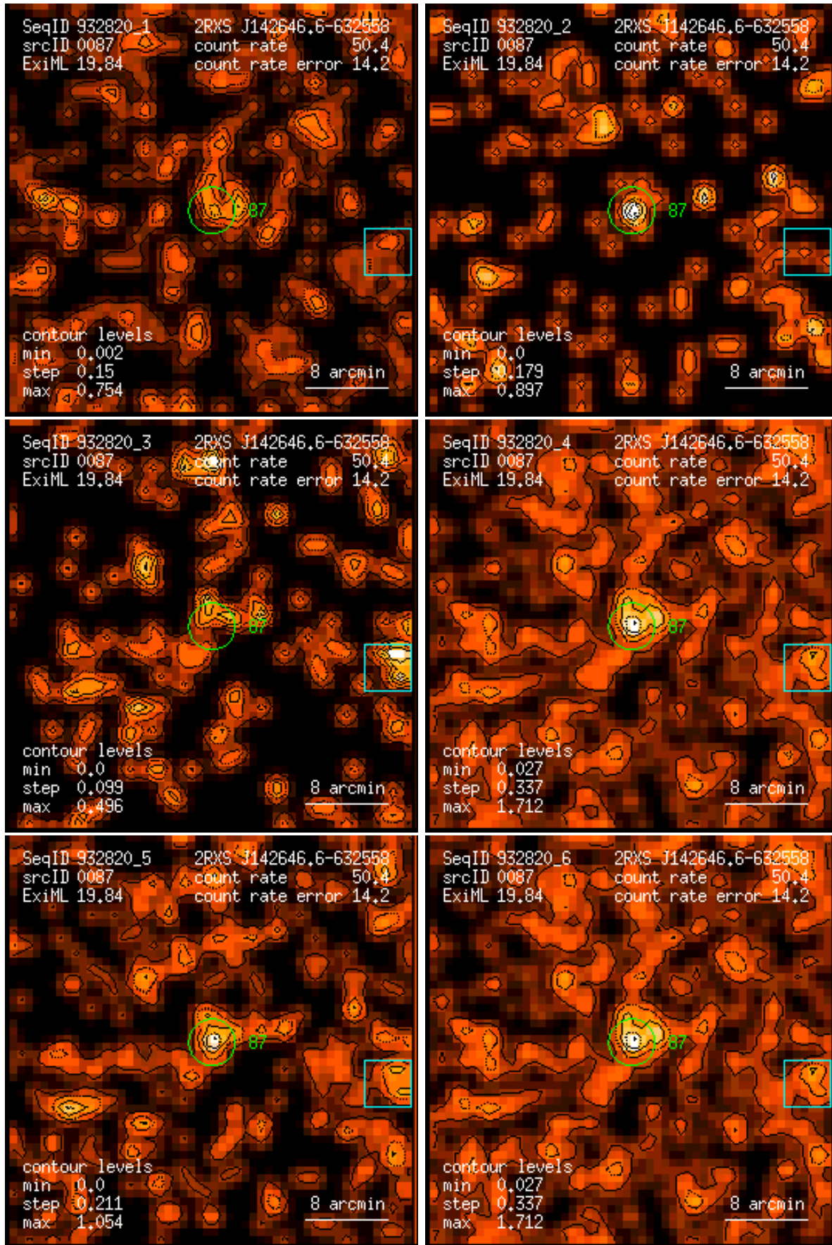
Figure 87: RASS 932820: detection 0087: band rate images, Gaussian filter: (1) PSPC channels 11 – 41, (2) 52 – 90, (3) 91 – 201, (4) 11 – 235, (5) 52 – 201, (6) 11 – 201. Broad band rates in counts/ks. Band rate contour levels in counts/ks/arcmin 2 .
